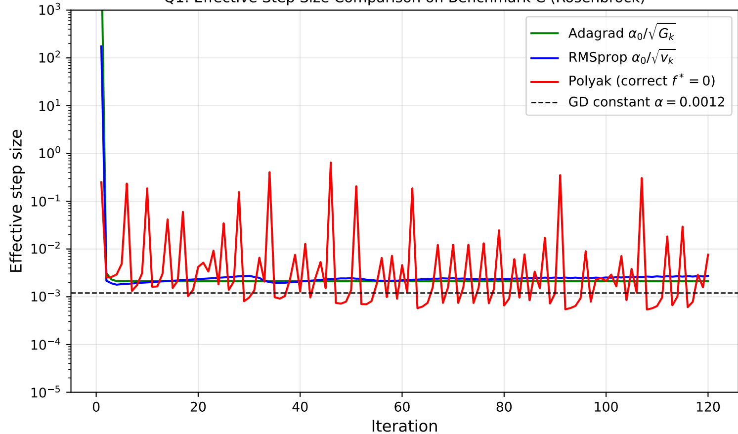
Q1: Effective Step Size Comparison on Benchmark C (Rosenbrock)
