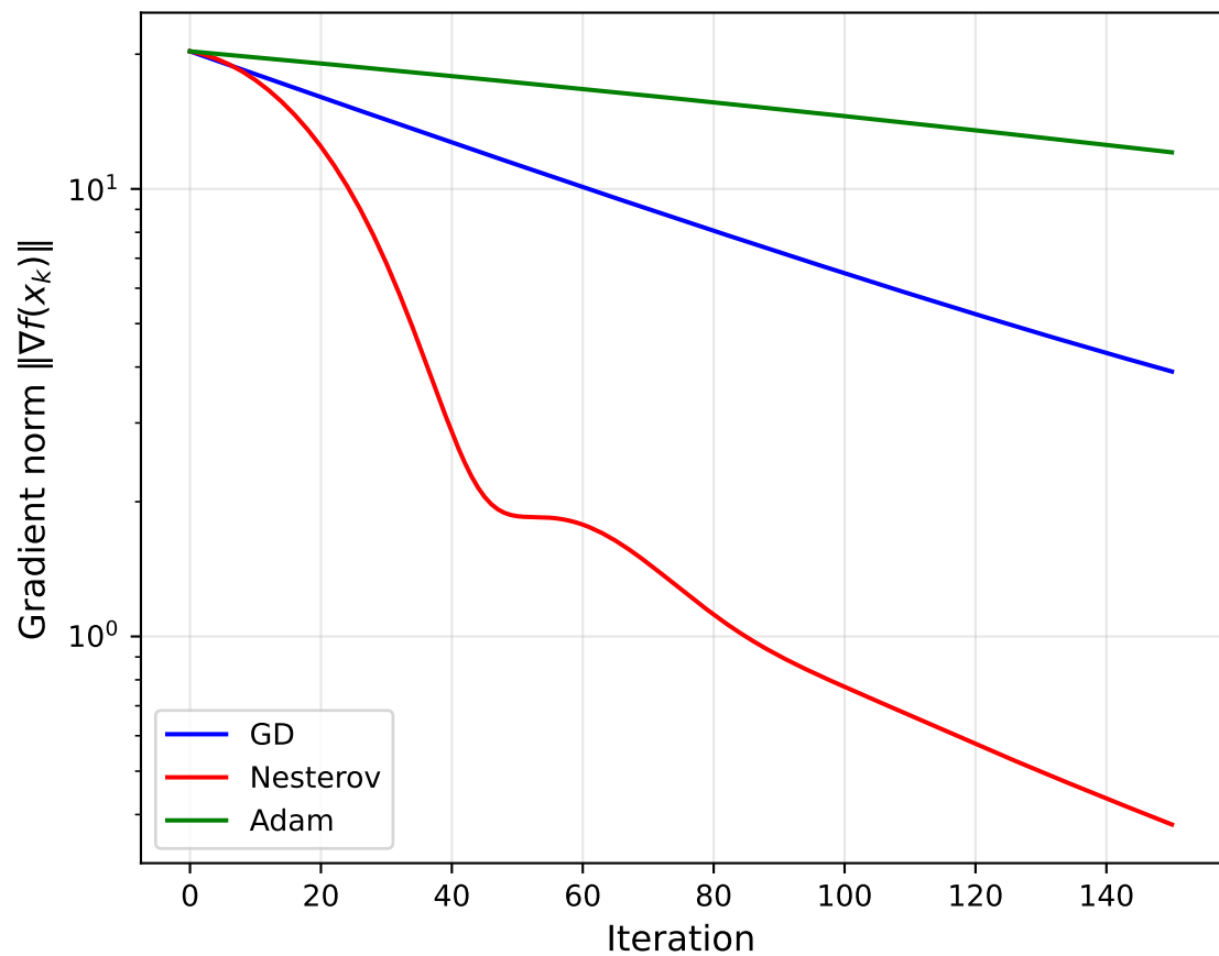
Q2: Gradient Norm Evolution on Benchmark C (Rosenbrock)
