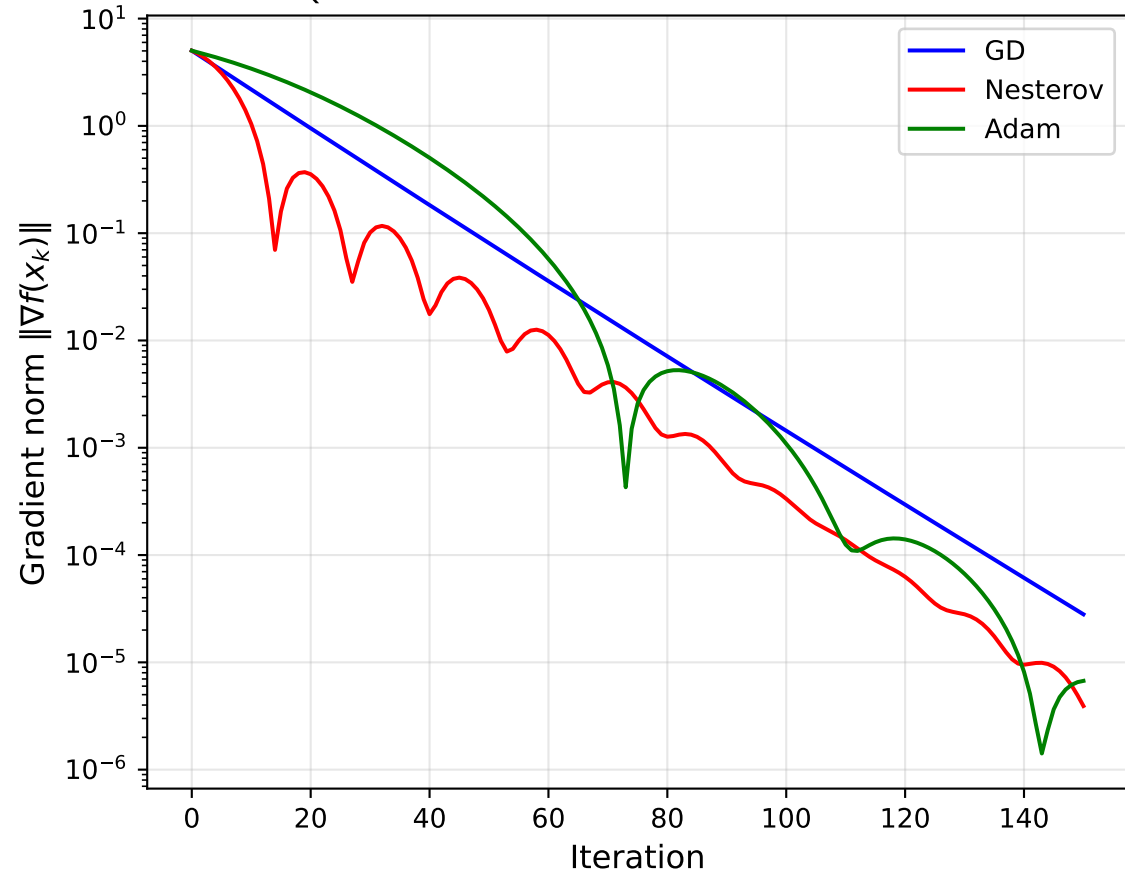
Q2: Gradient Norm Evolution on Benchmark A
