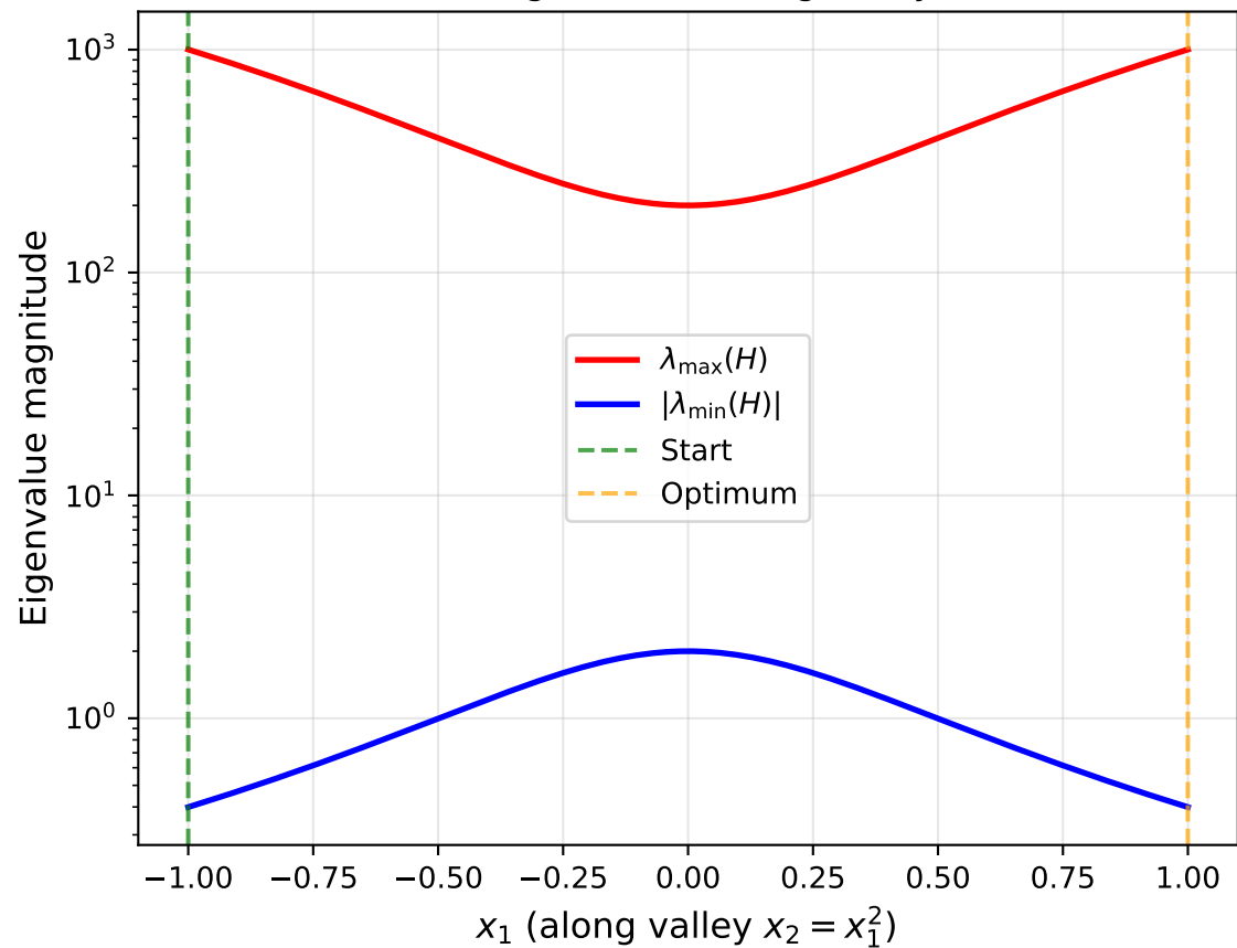
Hessian Eigenvalues Along Valley Floor
