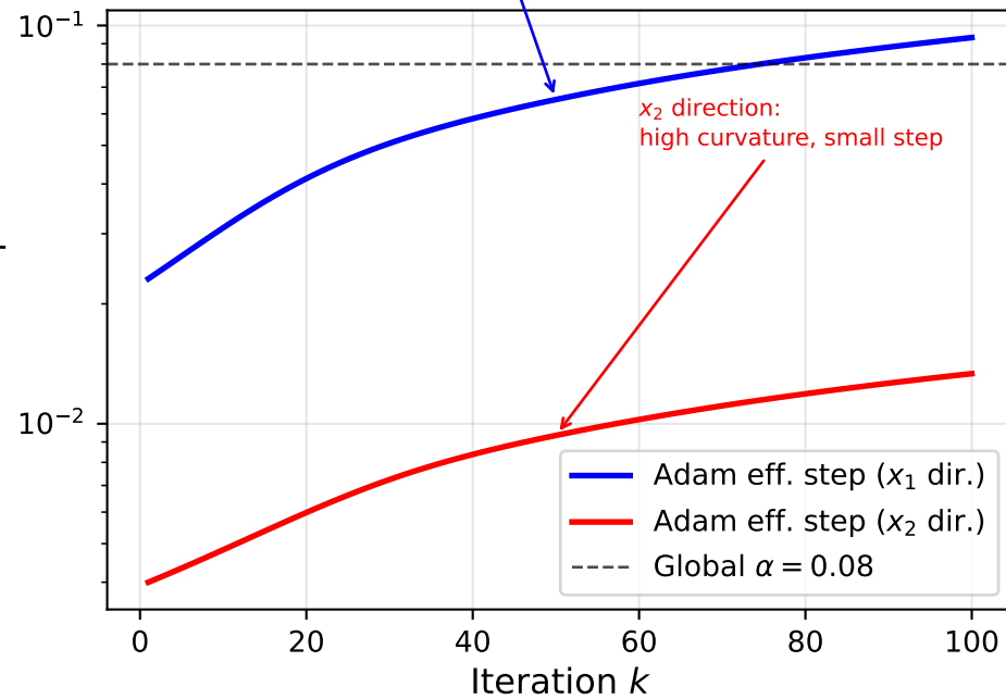
Adam Per-Coordinate Steps (Benchmark B)
