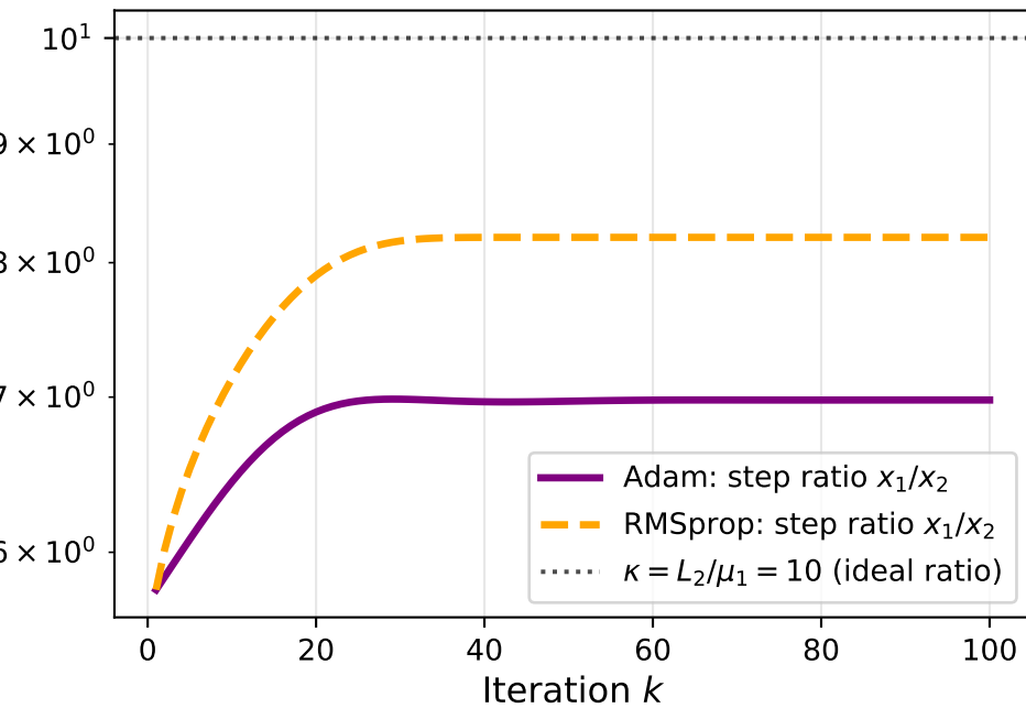
Step Ratio vs Ideal \kappa Ratio (ideal = 10 for Benchmark B)
