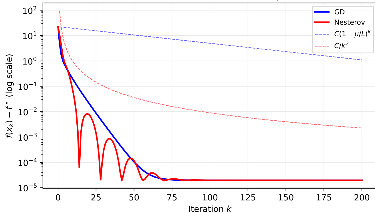
GD vs Nesterov Convergence on Benchmark B with Theoretical Rate Overlays
