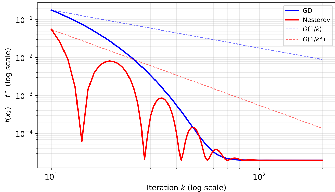
Log--Log Convergence Plot (slope = -1 for GD, = -2 for Nesterov)
