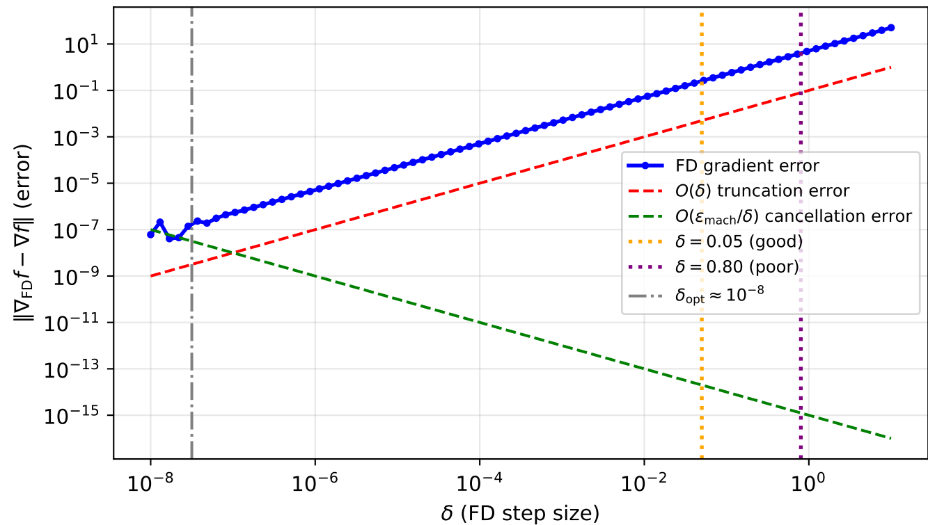
Finite Difference Gradient Error vs \delta at x = (0, 3) on Benchmark B
