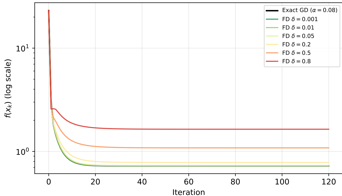
FD Gradient Descent: Effect of \delta on Benchmark B (Greener = smaller \delta , better approximation)
