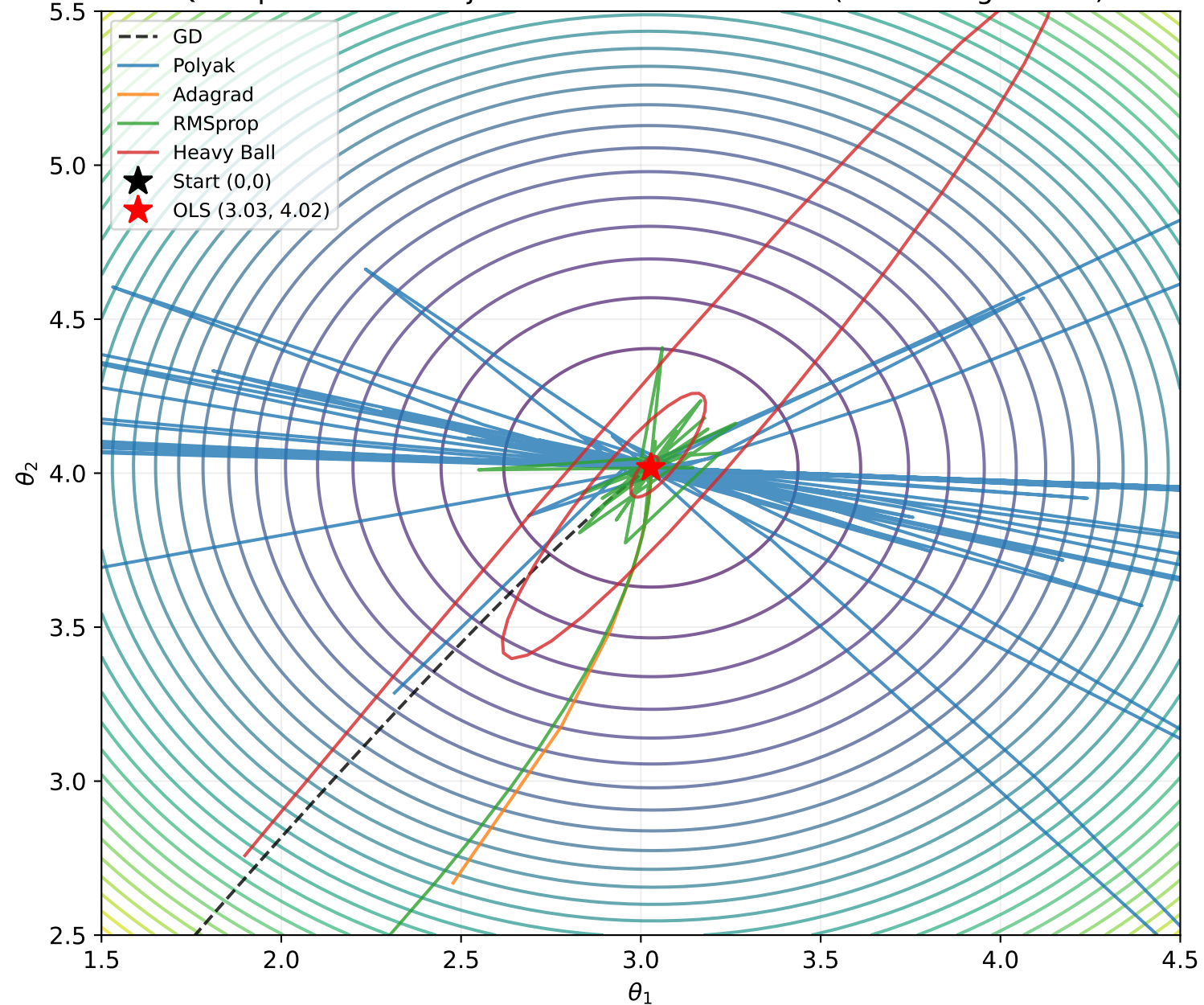
Q1: Optimisation Trajectories — Benchmark A (Linear Regression)
