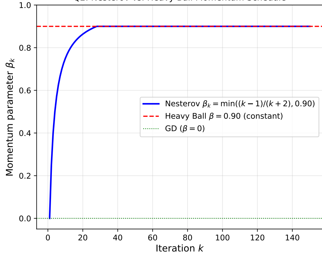
Q2: Nesterov vs. Heavy Ball Momentum Schedule
