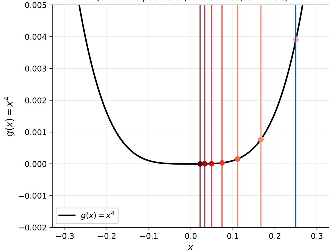
Q3: Iterate positions (Newton=red, GD=blue)
