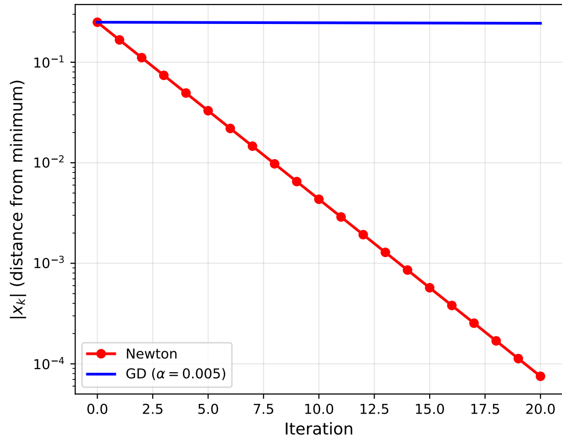
Q3: Newton vs GD on g(x) = x^4
