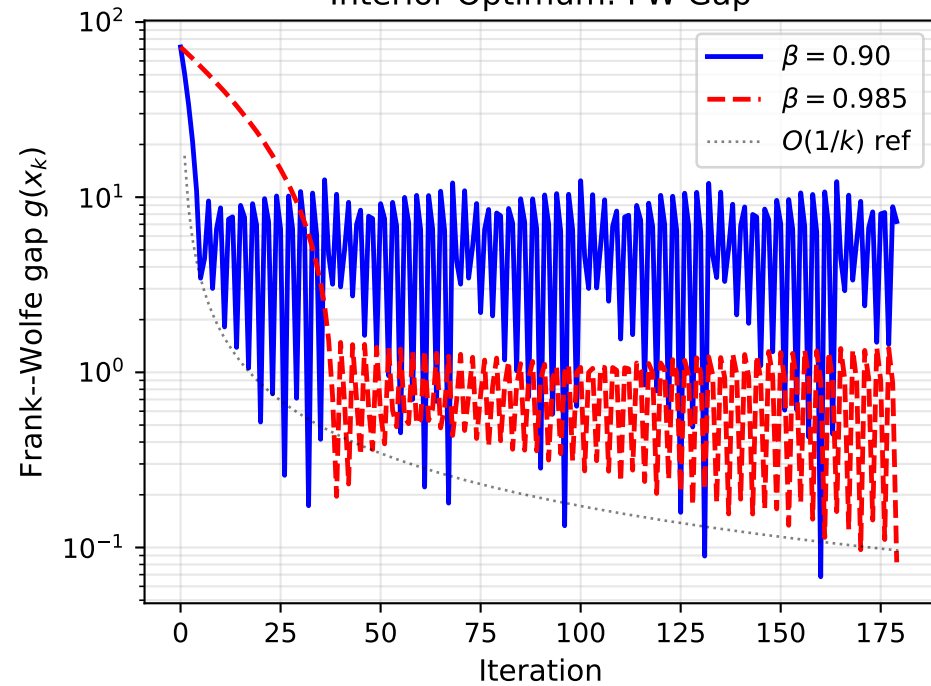
Interior Optimum: FW Gap
