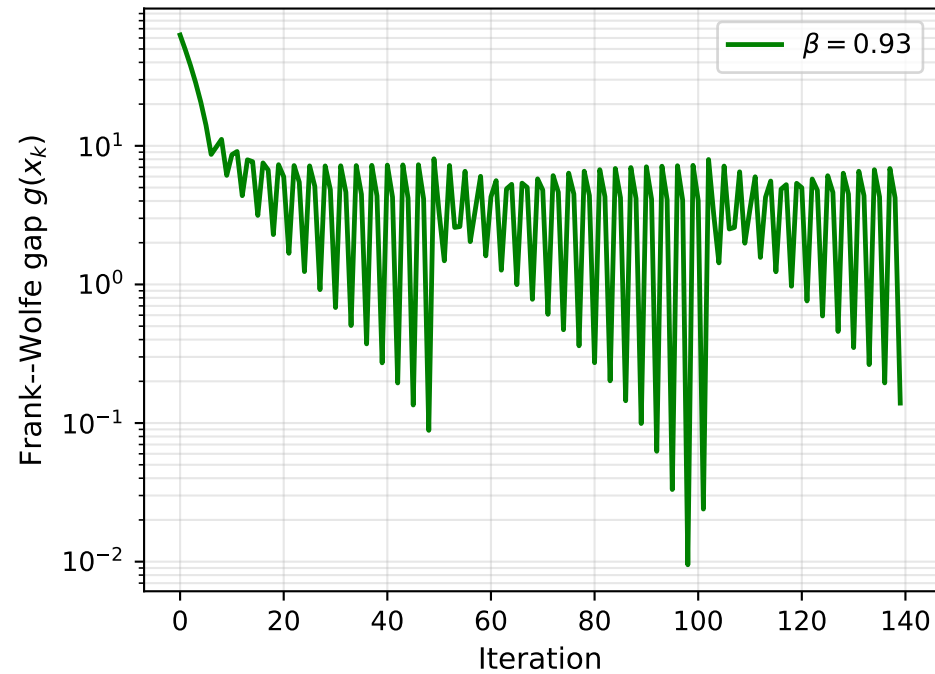
Boundary Optimum: FW Gap
