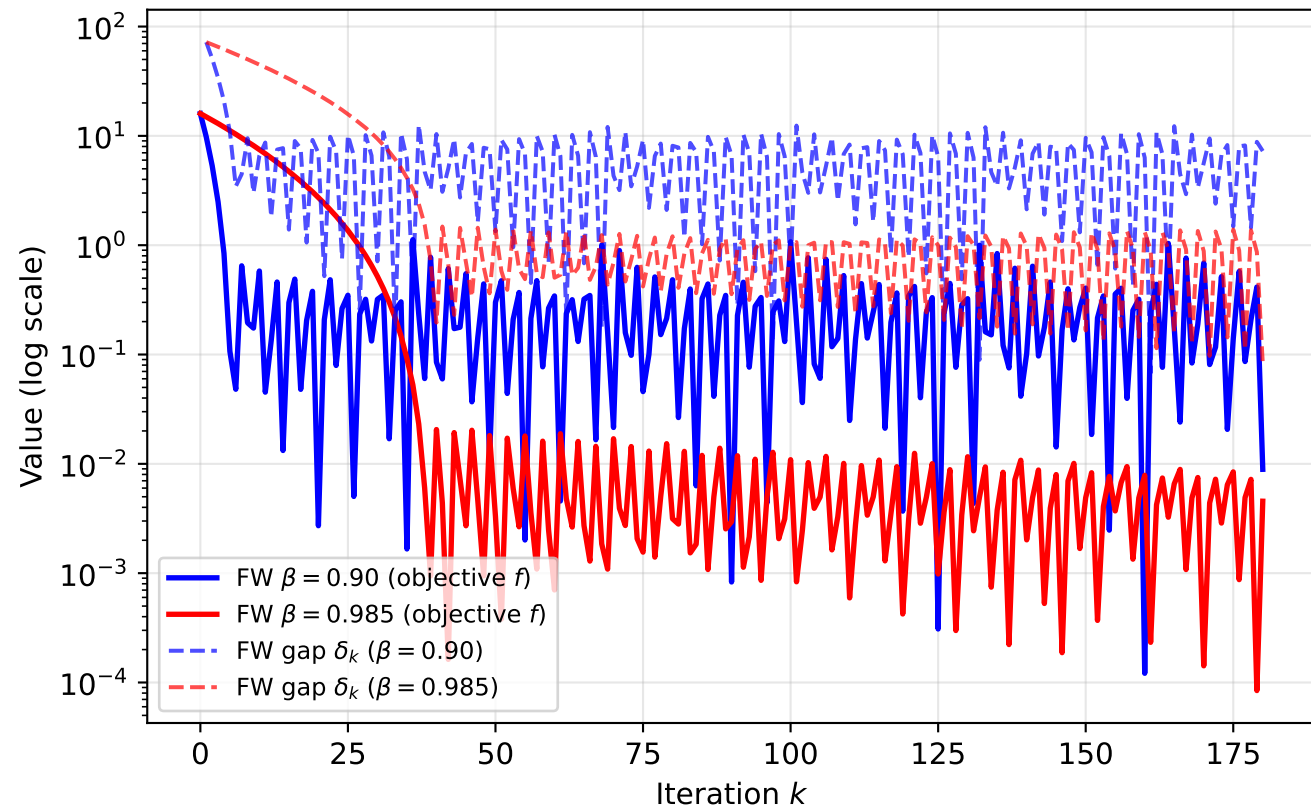
Q6-II: Objective and Frank--Wolfe Gap vs Iteration (Interior optimum, f = (x_1 - 1)^2 + (x_2 - 5)^2 )
