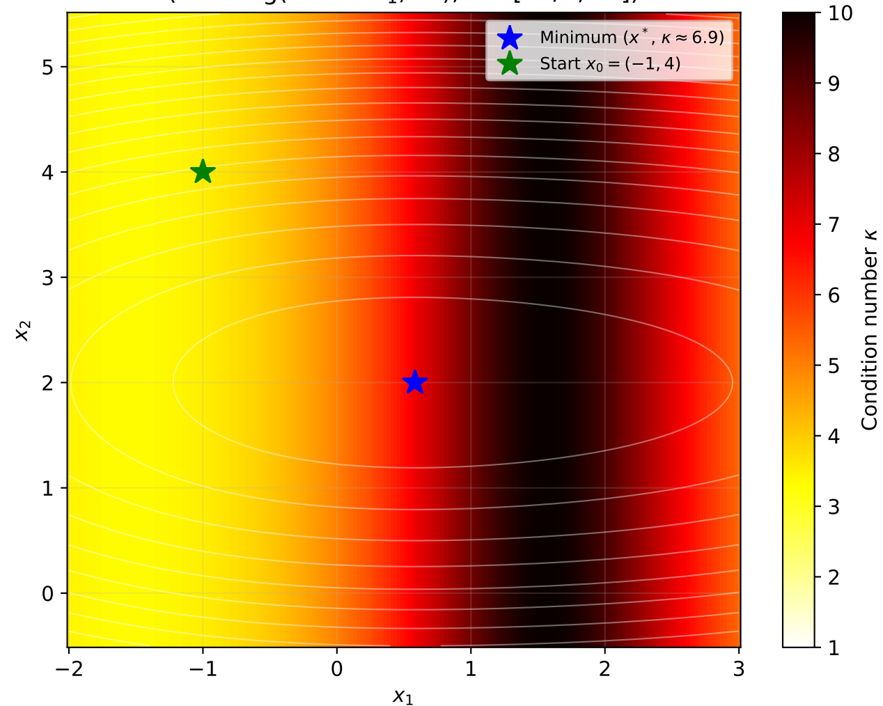
Benchmark B: Hessian Condition Number \kappa(x) Map ( H = \text{diag}(2 - \sin x_1, 10) , \kappa \in [10/3, 10] )
