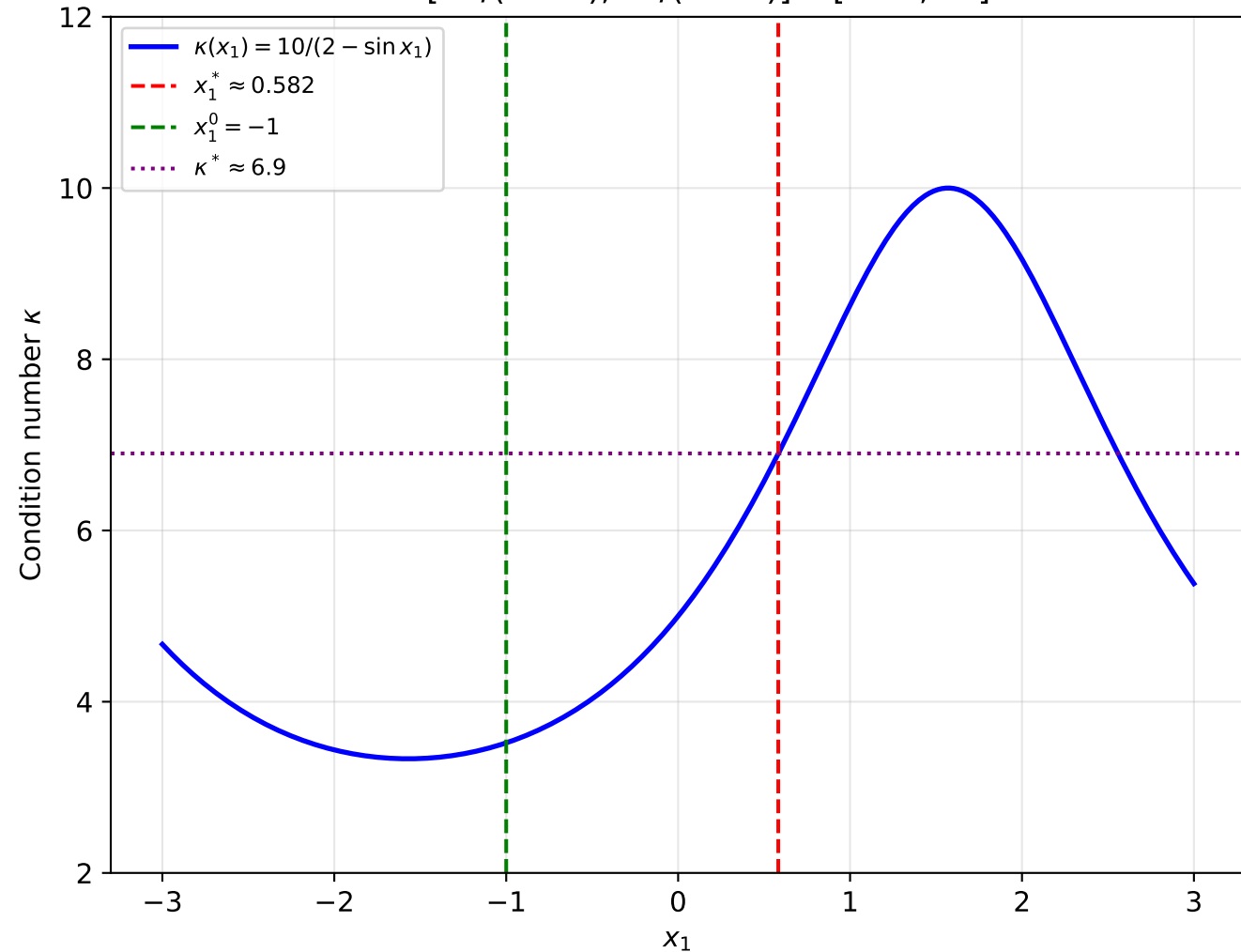
Benchmark B: \kappa Along x_2 = 2 (Valley Floor) \kappa \in [10/(2 + 1), 10/(2 - 1)] = [3.33, 10]
