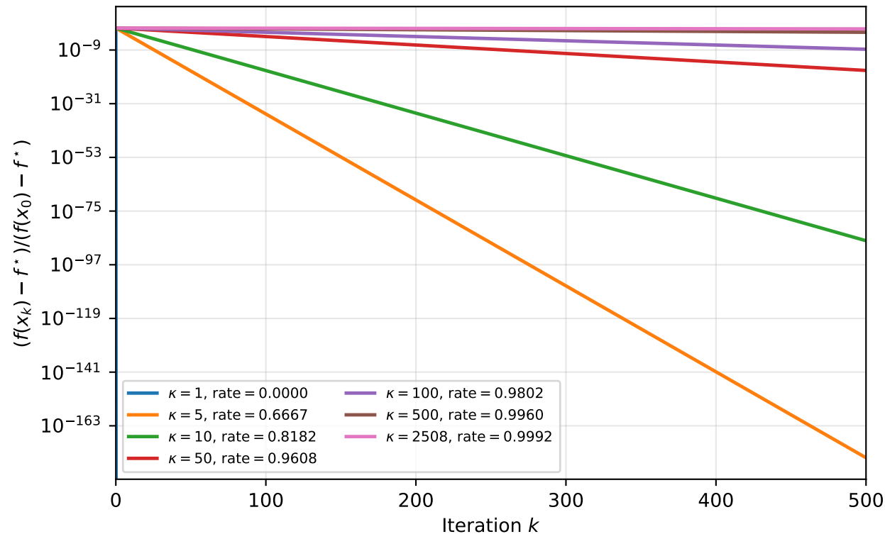
GD Convergence Rate vs Condition Number (optimal \alpha^* = 2/(\mu + L) )
