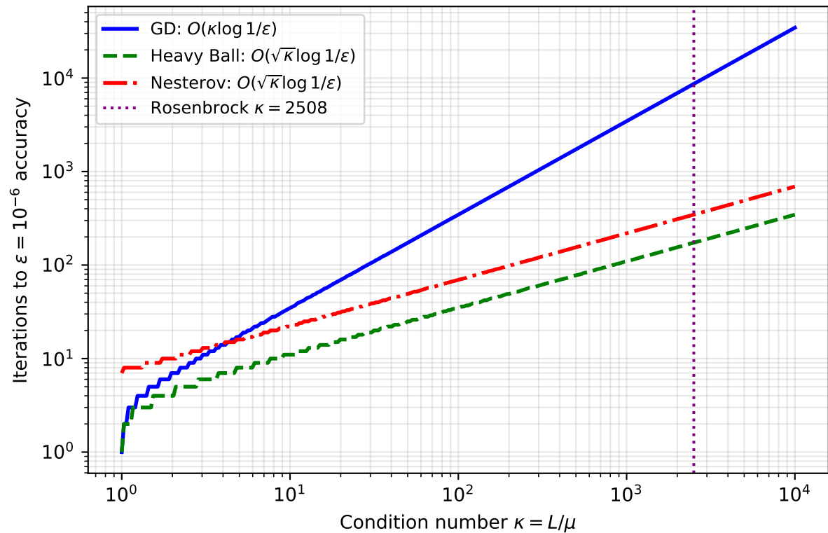
Iterations Required vs Condition Number (to reach \varepsilon = 10^{-6} accuracy)
