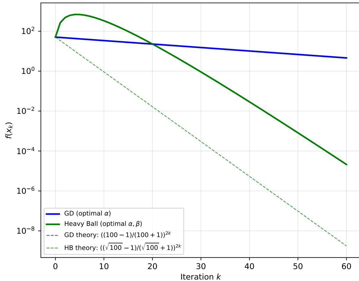
Convergence: GD vs HB ( \kappa = 100 ) HB converges \sqrt{\kappa} -times faster
