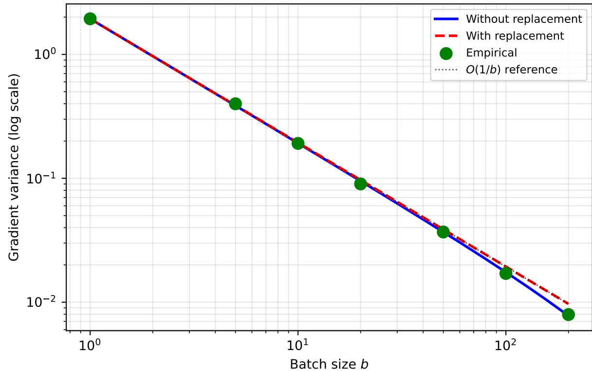
Gradient Variance vs Batch Size (log--log) W/R variance \propto 1/b ; W/O/R variance \rightarrow 0 at b = m
