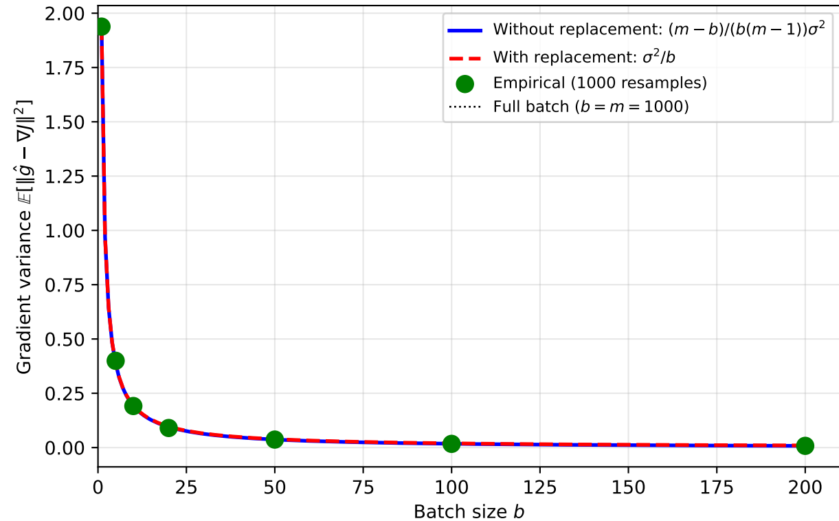
Mini-Batch SGD Gradient Variance vs Batch Size (Benchmark A, m = 1000 , d = 2 )
