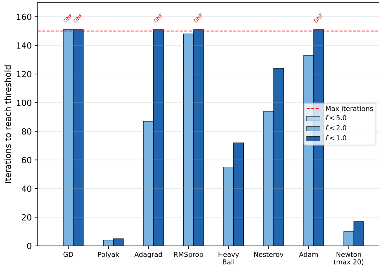
Iterations-to-Threshold on Benchmark C
