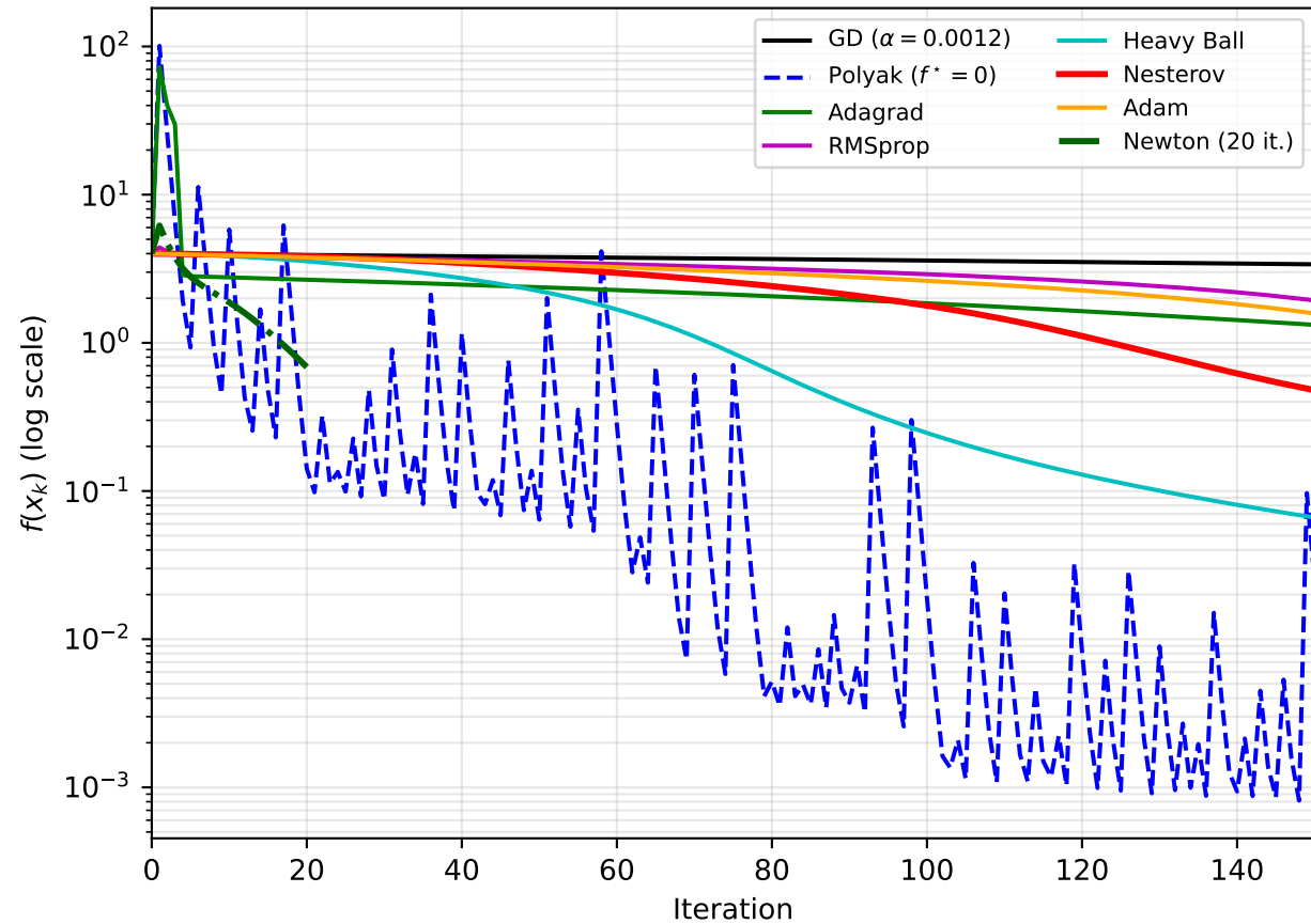
All Methods on Benchmark C (Rosenbrock)
