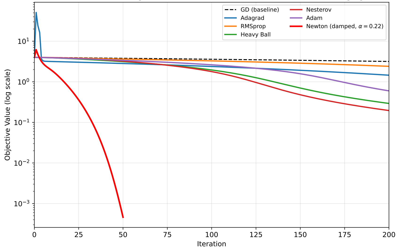
All Methods: Convergence on Benchmark C (Rosenbrock, most challenging)
