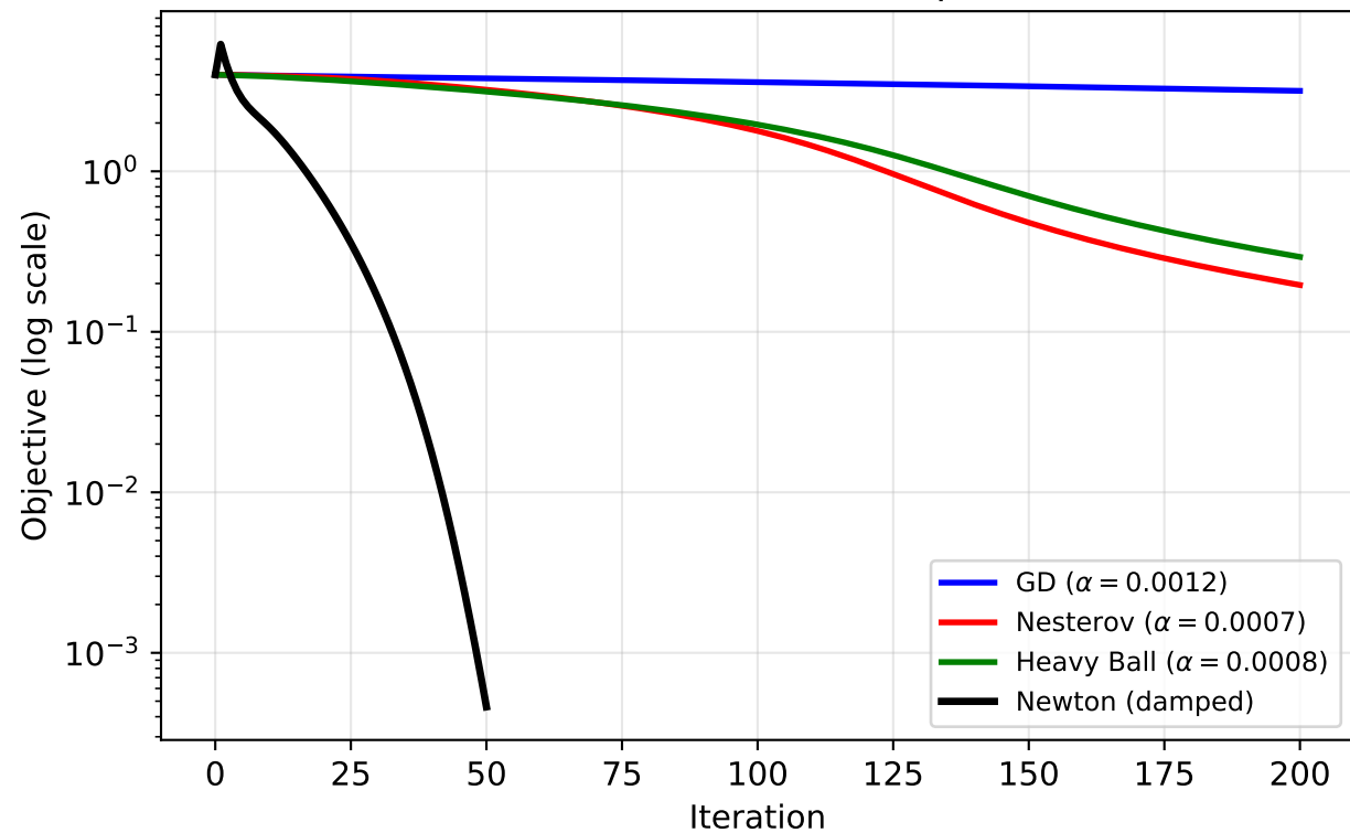
Benchmark C (Rosenbrock): Empirical Convergence (non-convex, \kappa \approx 2508 at optimum)
