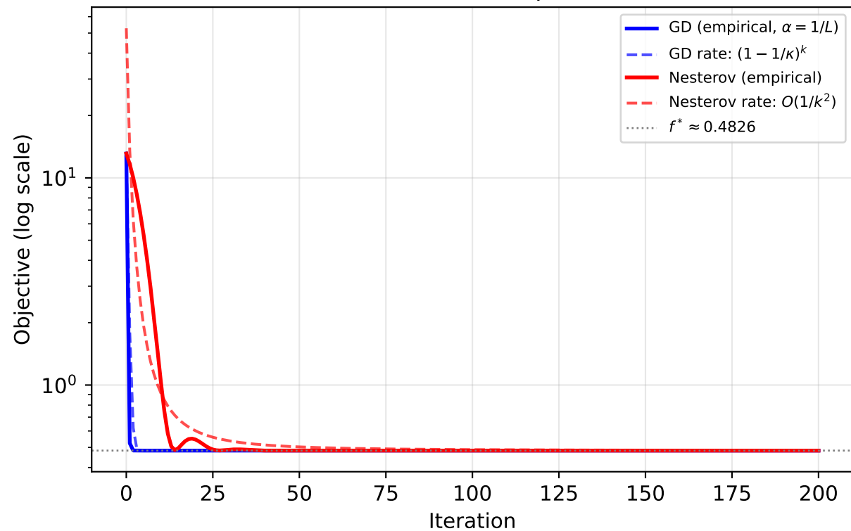
Benchmark A: Theoretical vs Empirical Rates ( \kappa = 1.12 , L = 1.033 , \mu = 0.925 )
