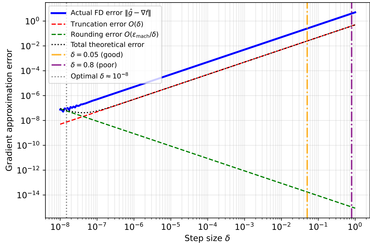
Q4: Finite Difference Approximation Error vs Step Size \delta
