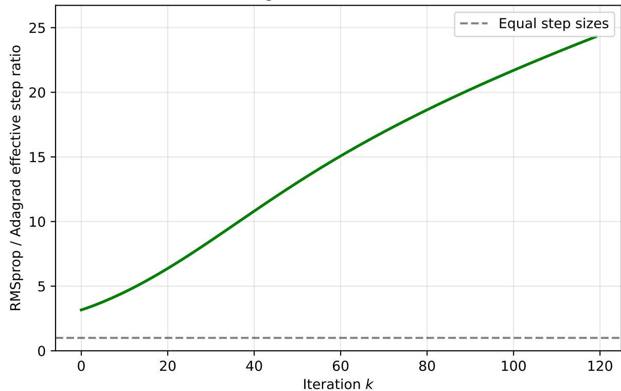
Step Size Ratio: RMSprop recovers faster when gradients become small
