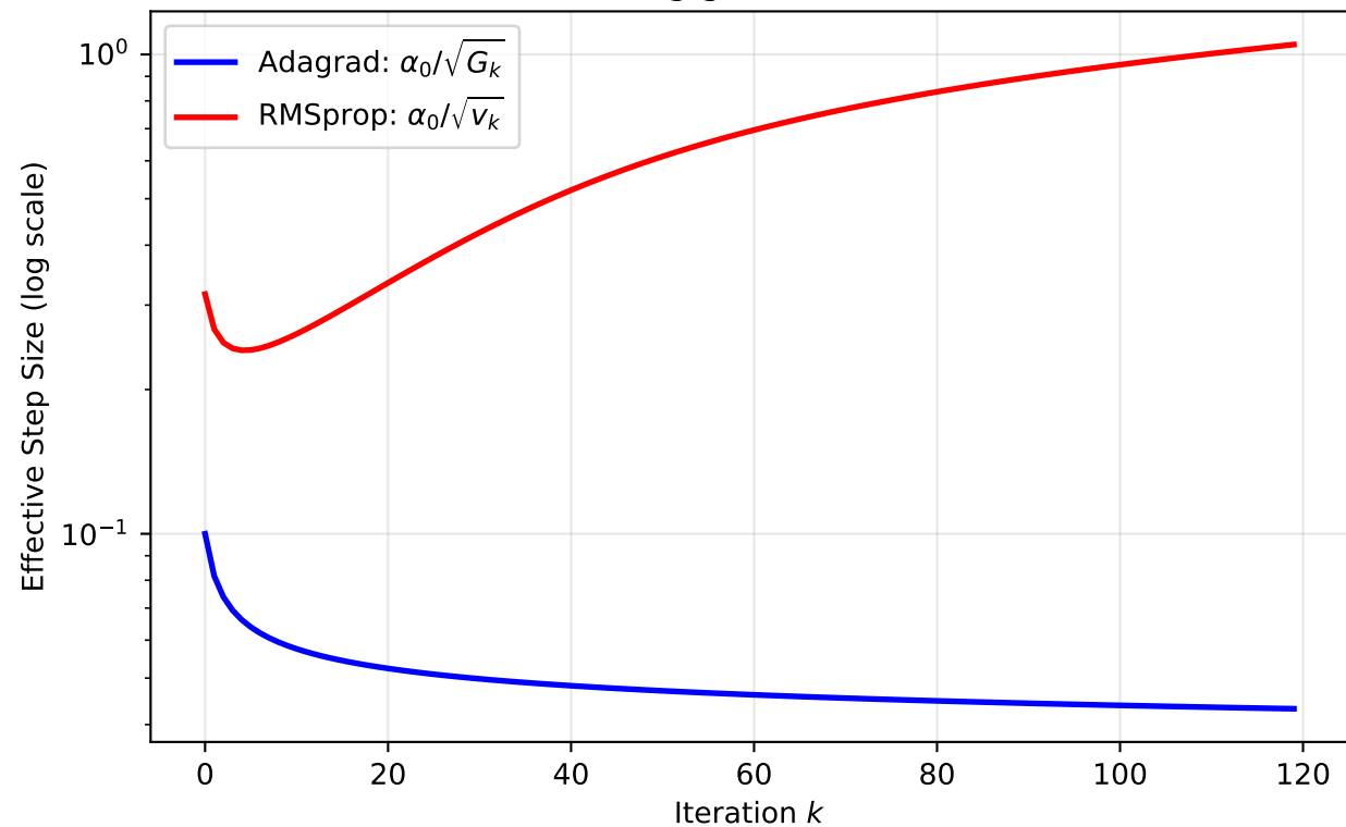
Adagrad vs RMSprop: Effective Step Evolution (Decreasing gradient scenario)
