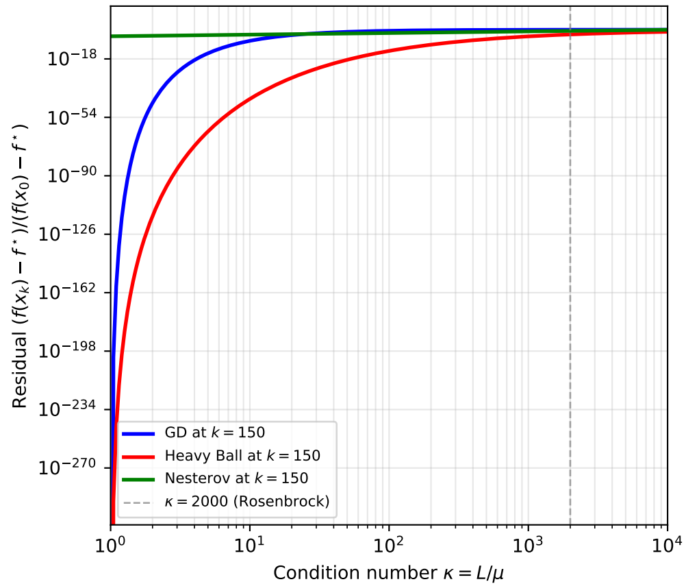
Residual after k = 150 iterations
