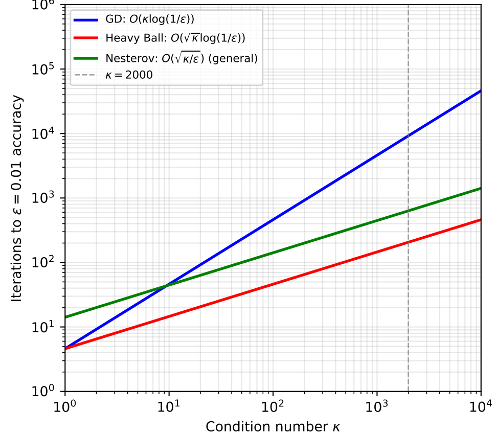
Iteration complexity vs \kappa ( \varepsilon = 0.01 )
