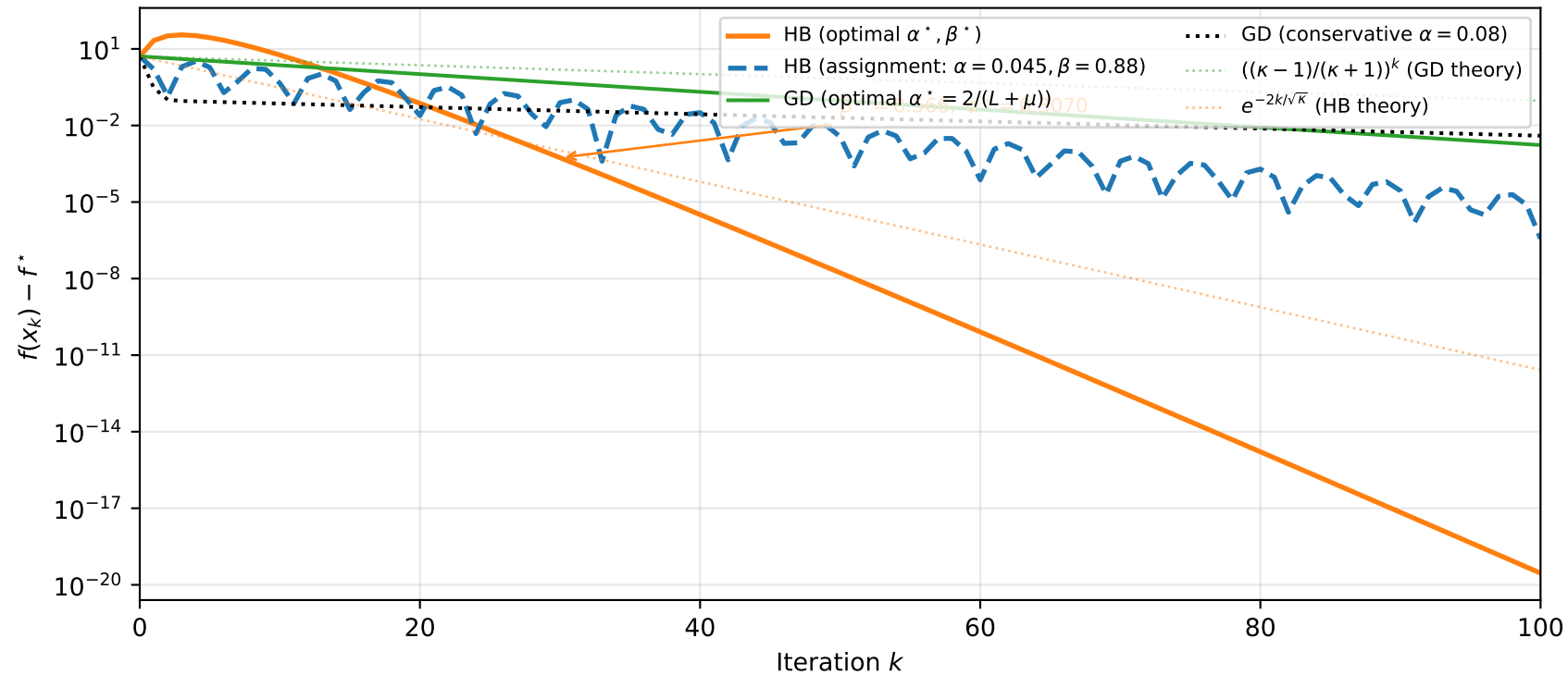
Heavy Ball: Optimal vs Experimental Parameters (Synthetic quadratic, \kappa = 50 , \mu = 0.2 , L = 10.0 )
