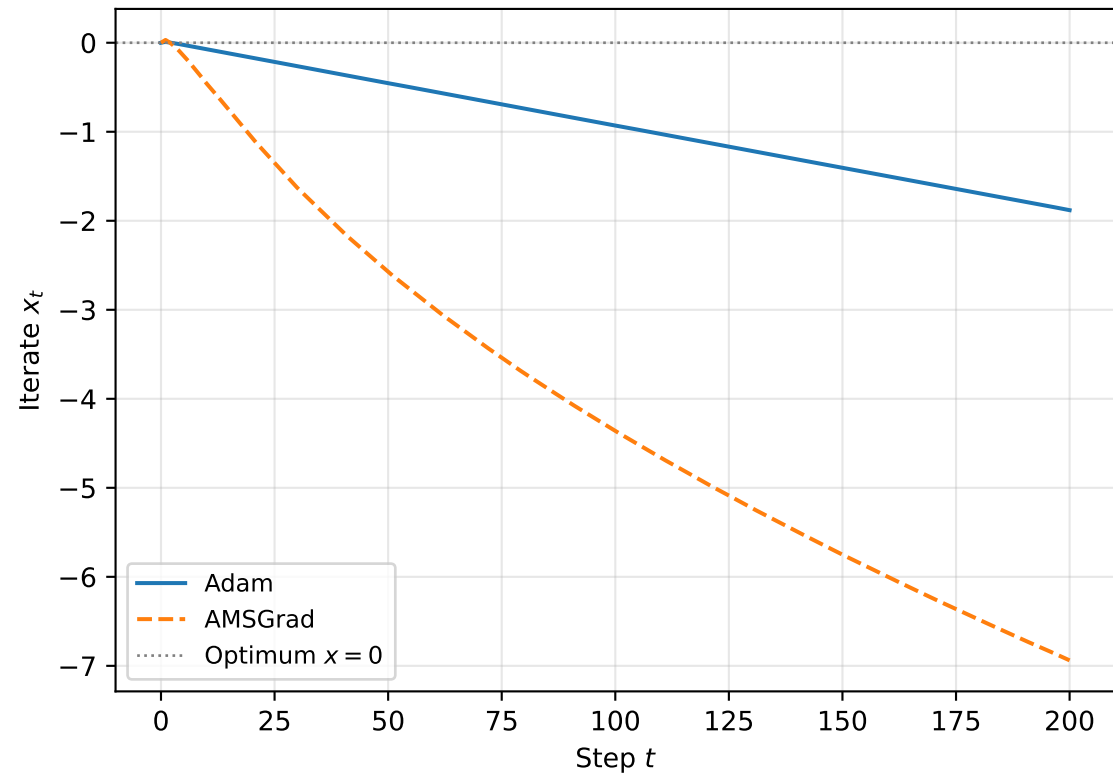
Adam vs AMSGrad: Adversarial Gradient ( C = 100 )
