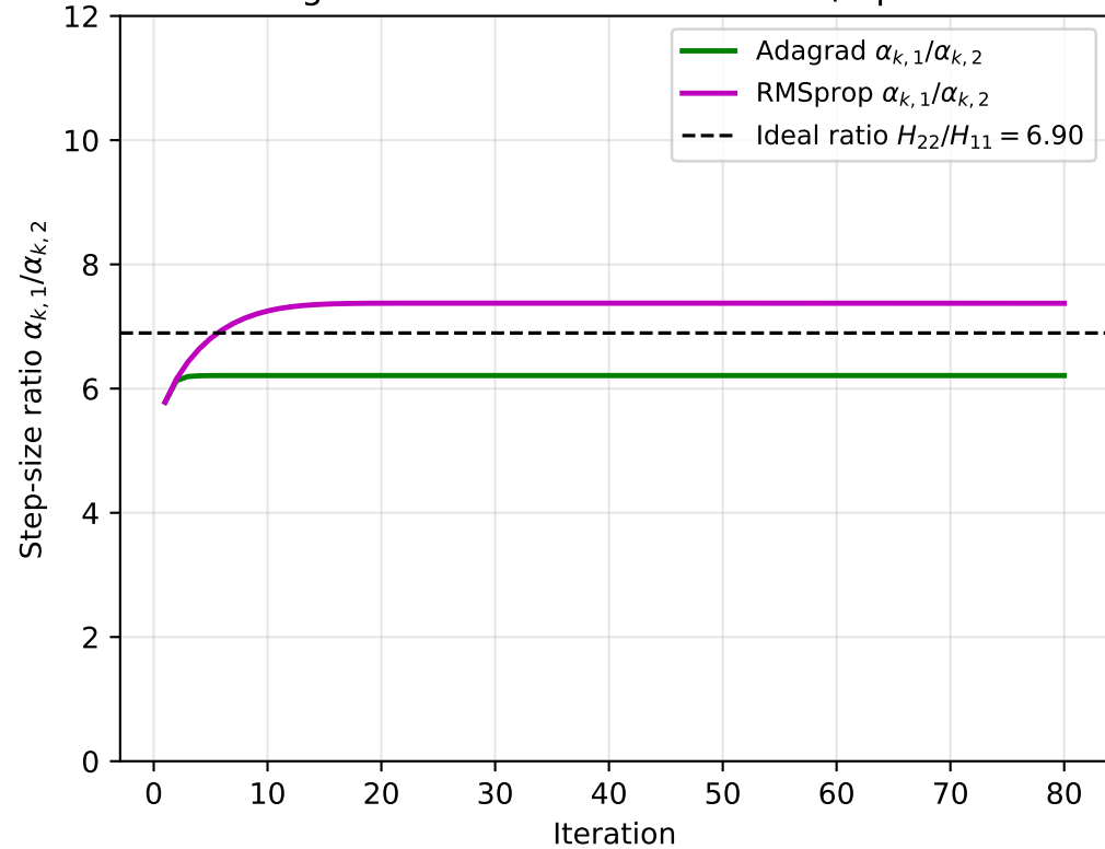
Diagonal Preconditioner Ratio vs. Optimal
