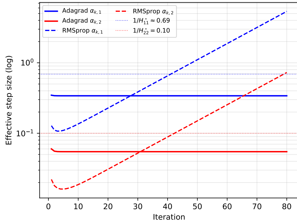
Adaptive Steps vs. Inverse Hessian Diagonal (Bench. B)
