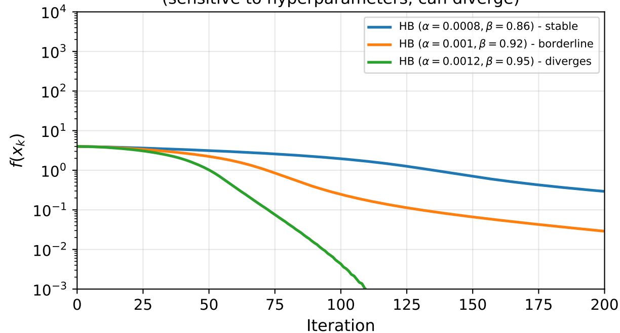
Heavy Ball on Rosenbrock (sensitive to hyperparameters, can diverge)
