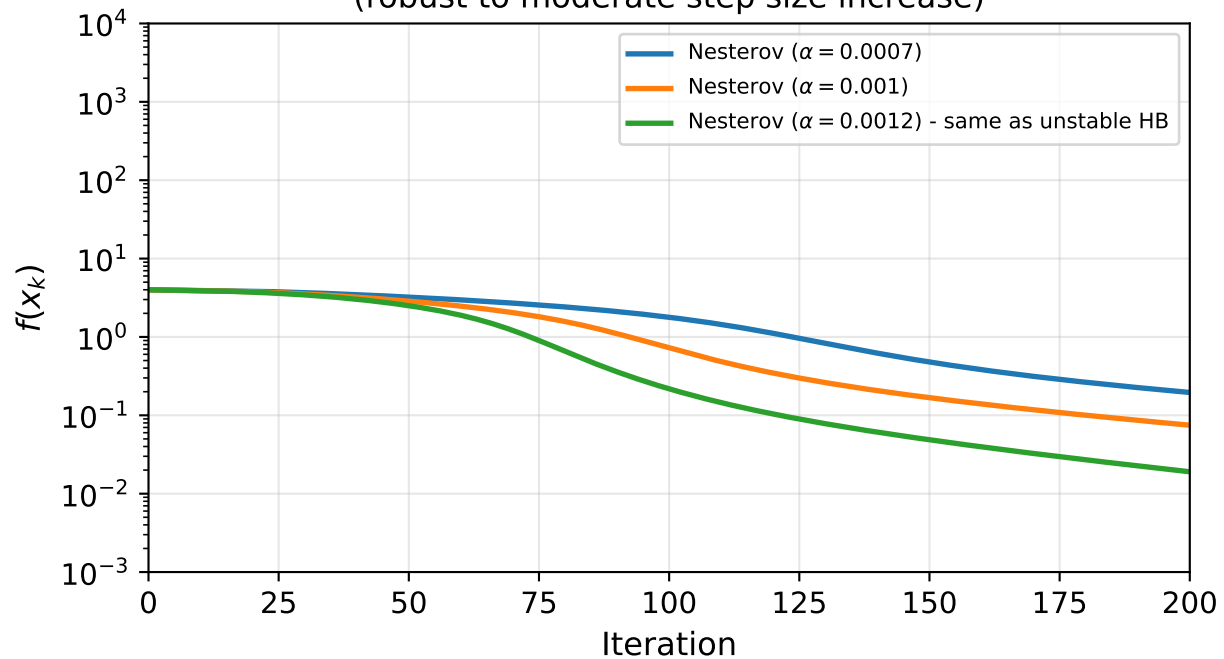
Nesterov Acceleration on Rosenbrock (robust to moderate step size increase)
