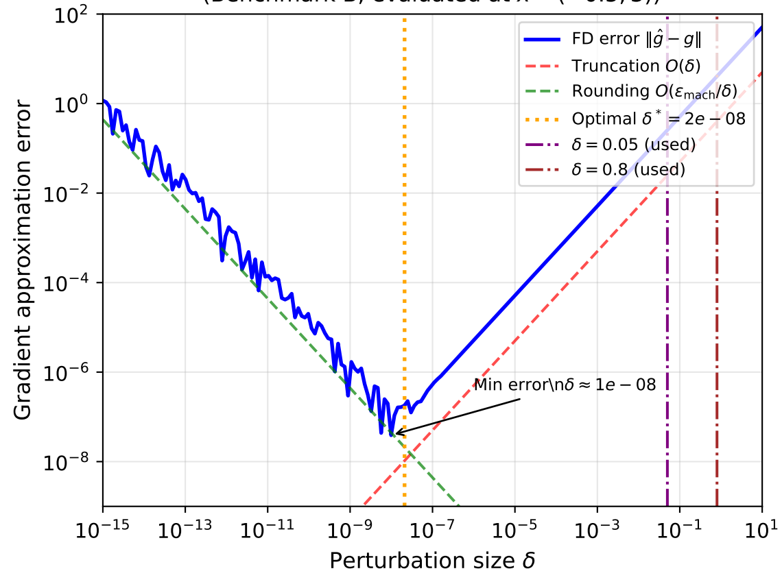
Forward FD Error: Truncation vs Rounding Tradeoff (Benchmark B, evaluated at x = (-0.5, 3) )
