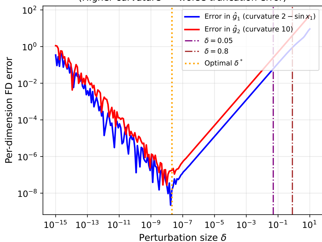
Per-Dimension FD Error (Higher curvature \Rightarrow worse truncation error)
