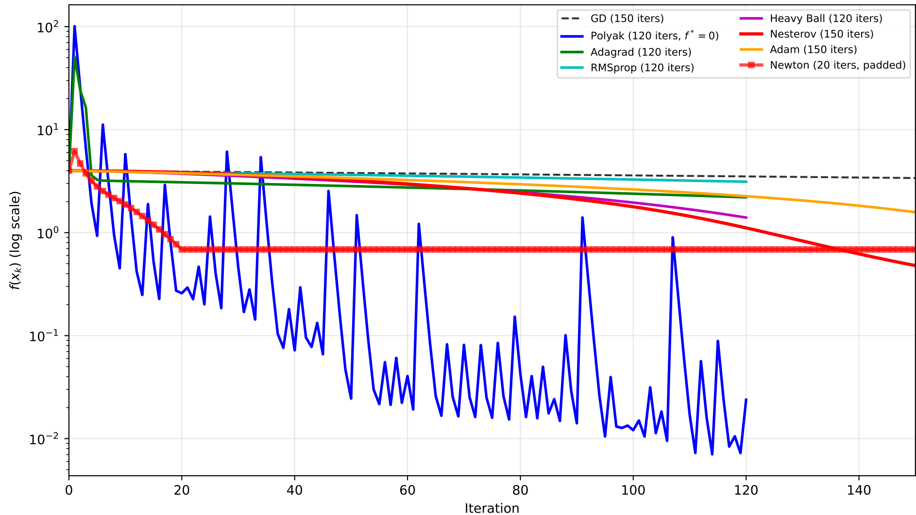
All Methods on Benchmark C (Rosenbrock, \kappa \approx 2508 )
