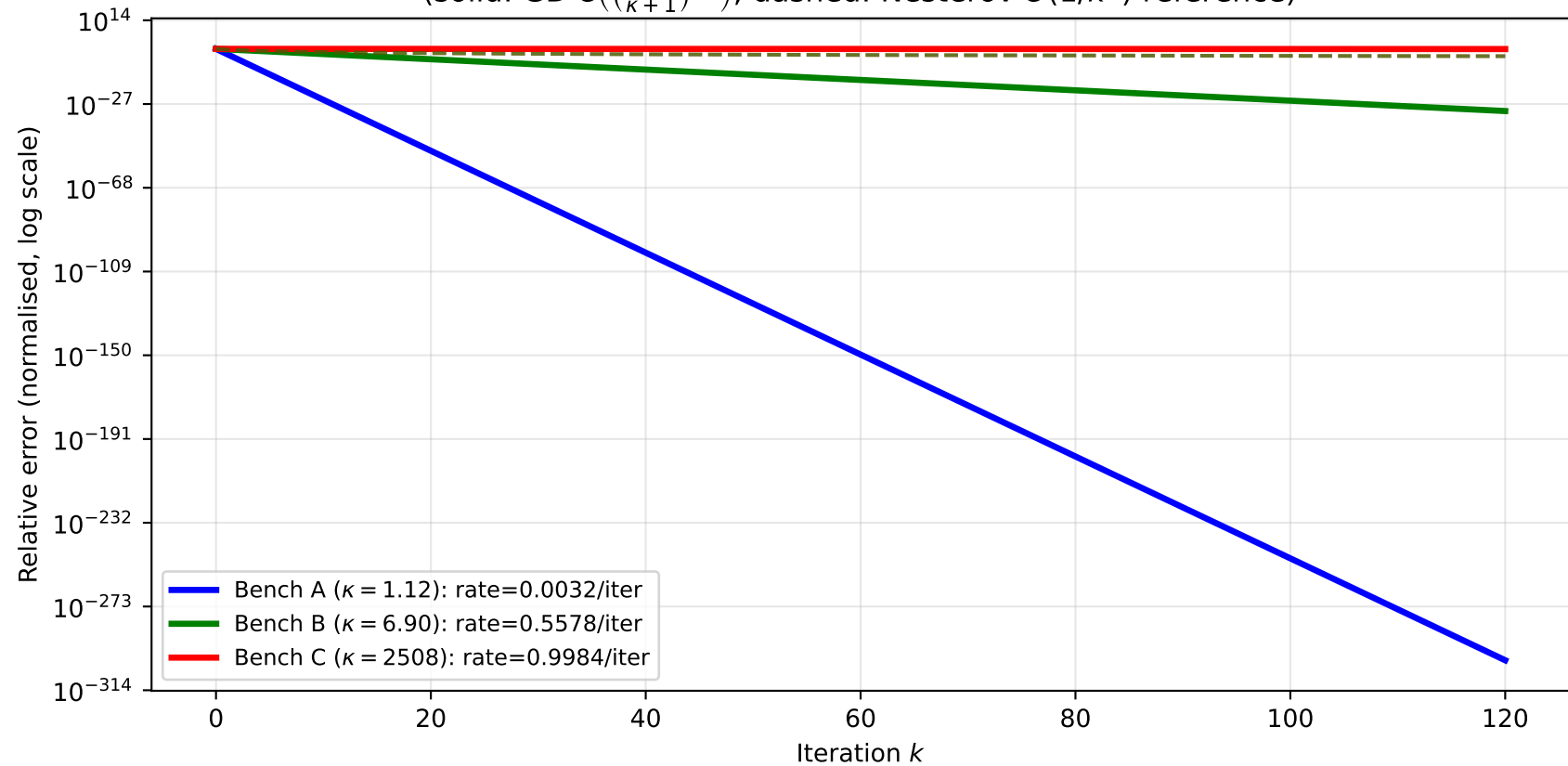
Gradient Descent Convergence Rate vs Condition Number (solid: GD O\left(\left(\frac{\kappa-1}{\kappa+1}\right)^{2k}\right) ; dashed: Nesterov O(1/k^2) reference)
