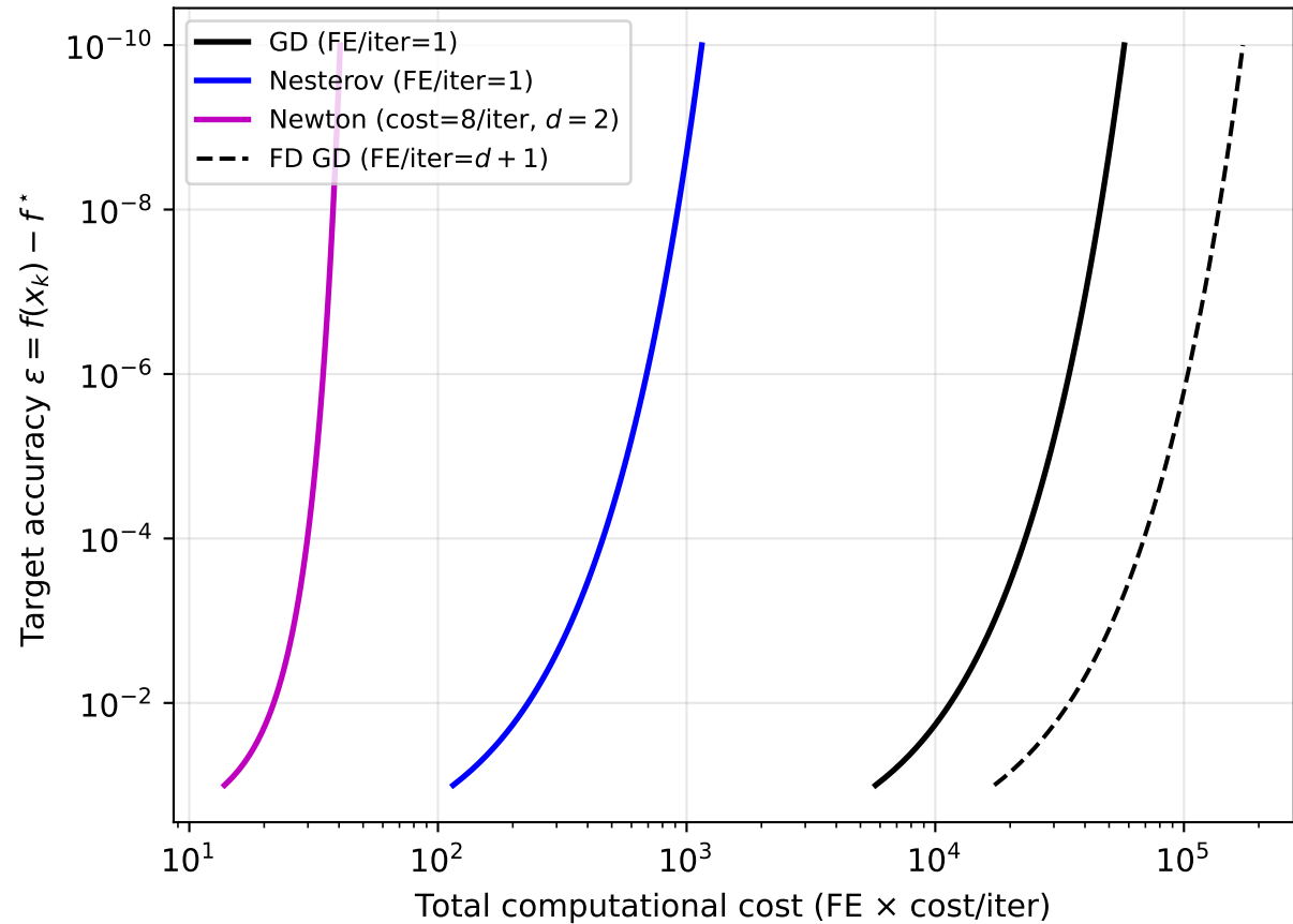
Total cost to reach \epsilon -accuracy ( d = 2 , \kappa = 2500 )
