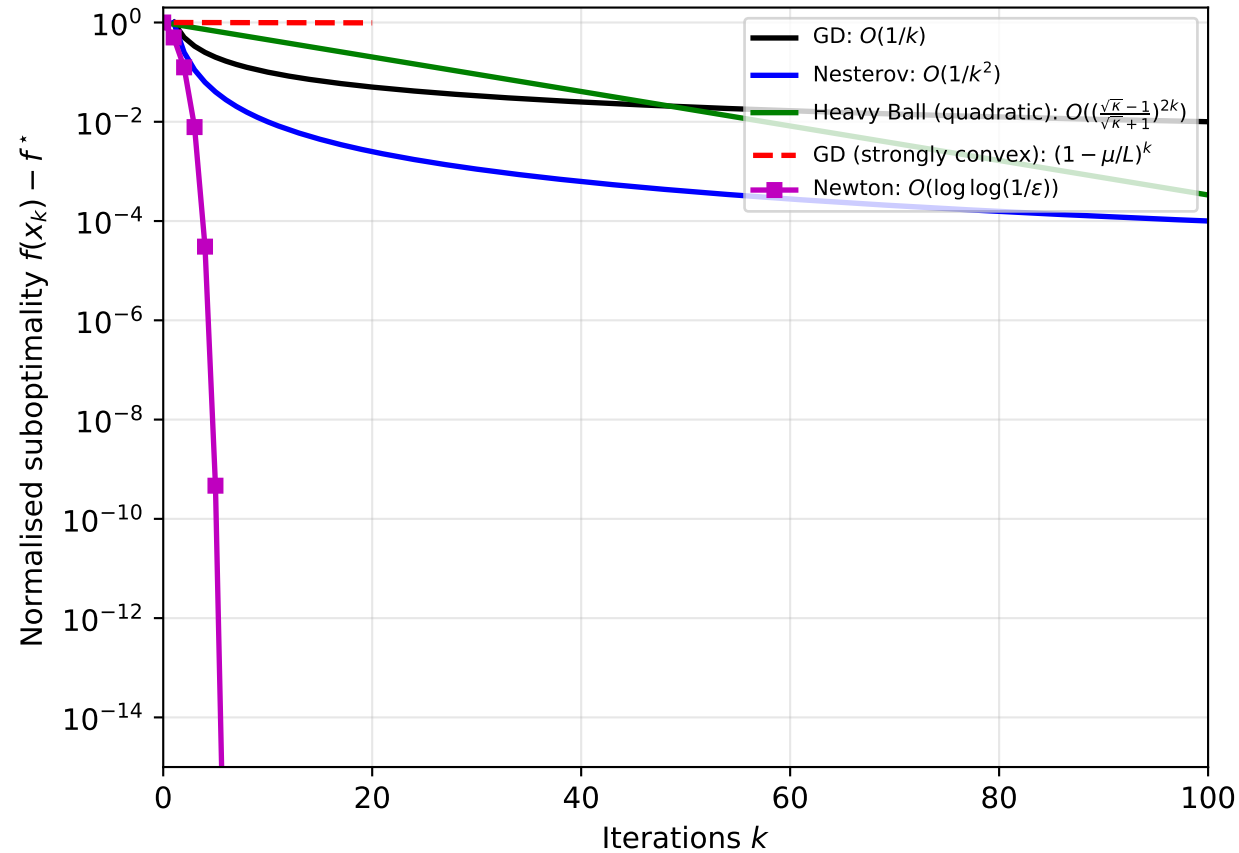
Theoretical convergence rates ( \kappa = 2500 , smooth strongly convex)
