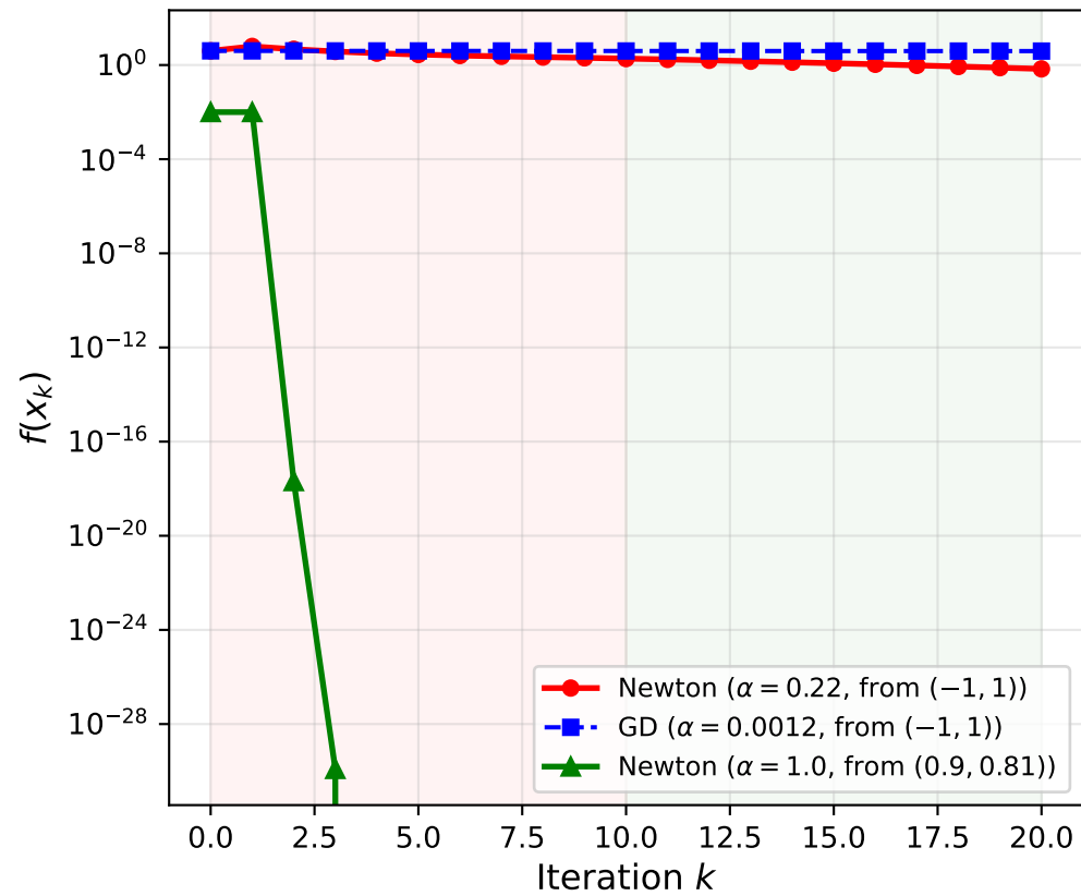
Newton: Global vs. Local Regime (Benchmark C)
