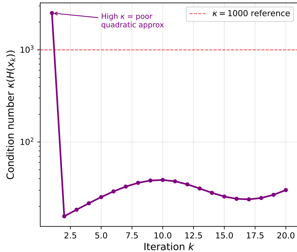
Hessian Condition Number Along Newton Path (Benchmark C)
