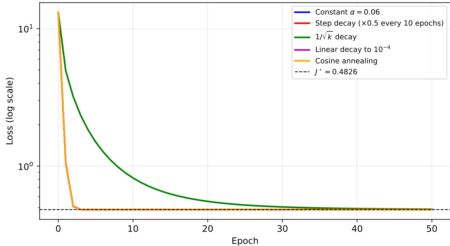
Q2: SGD Learning Rate Schedules Comparison (b=40, Benchmark A)
