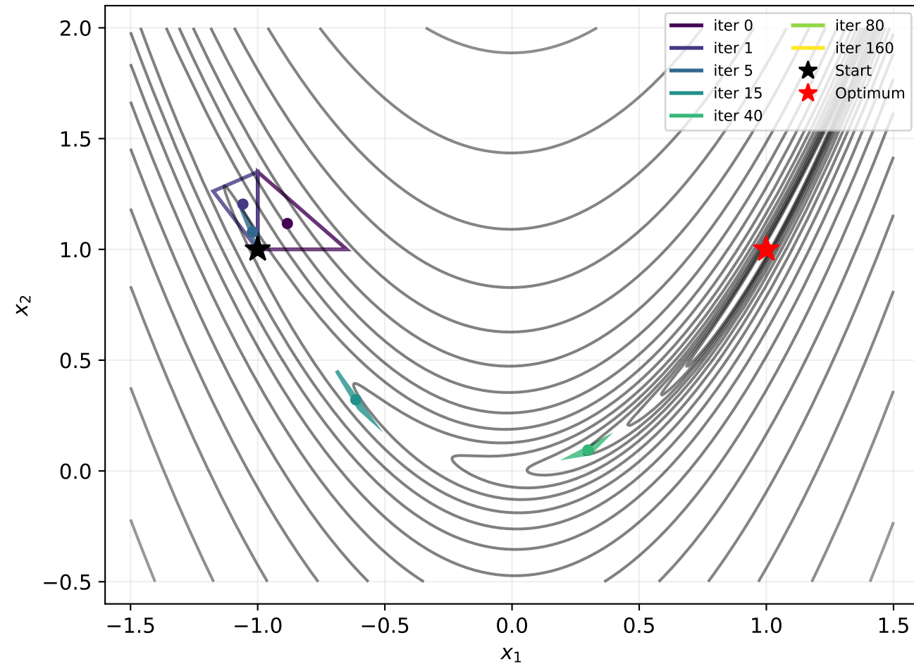
Q4B: Nelder--Mead Simplex Evolution (snapshots at selected iterations)
