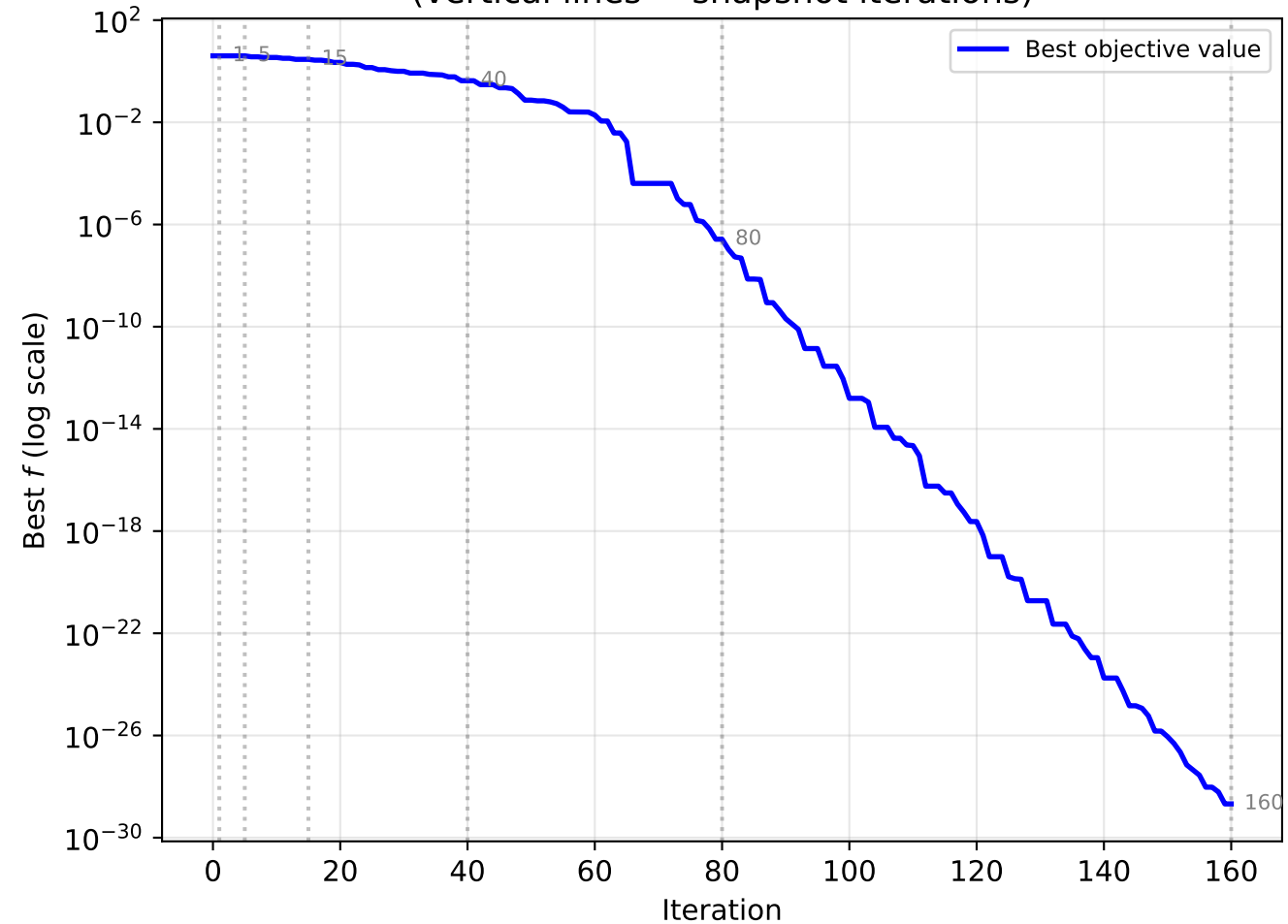
Q4B: Nelder--Mead Convergence (vertical lines = snapshot iterations)
