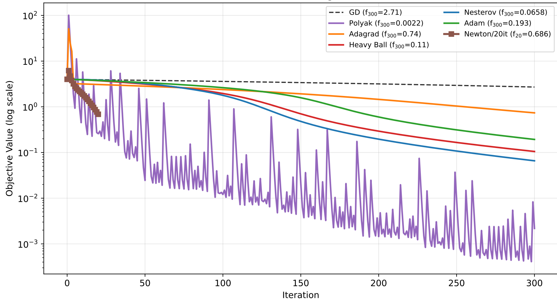
All Methods Compared on Rosenbrock Benchmark C (300 iterations, log scale)
