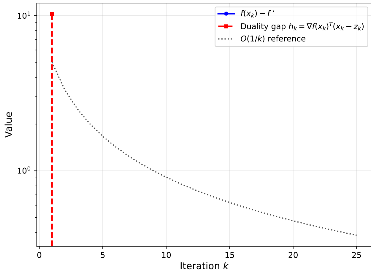
FW Convergence: Primal Gap vs. Duality Gap
