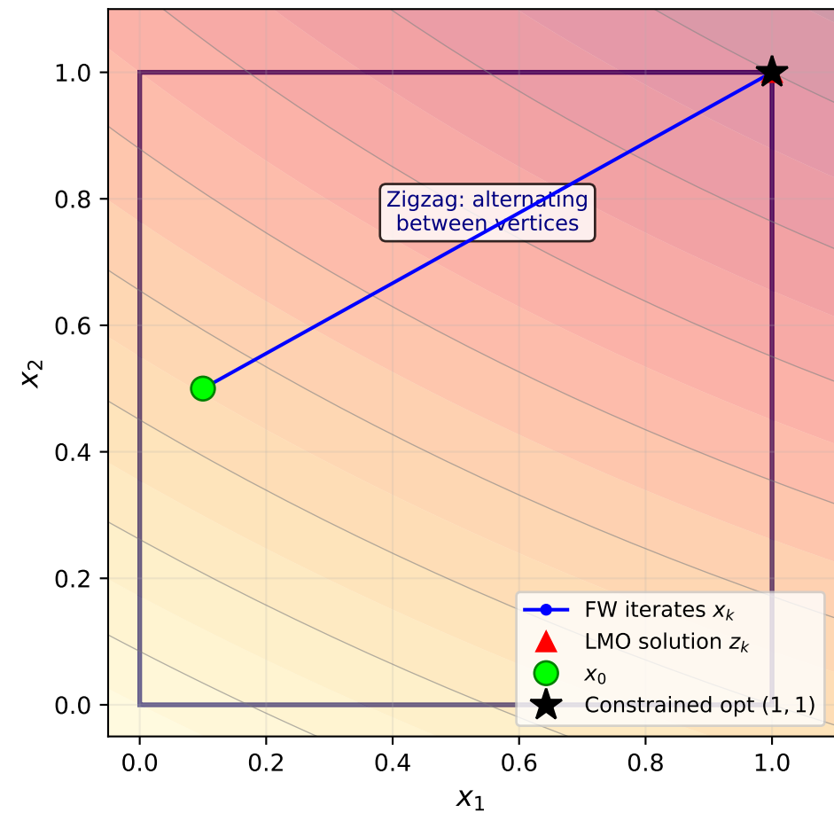
Frank--Wolfe Trajectory (FW with \gamma_k = 2/(k + 2) )
