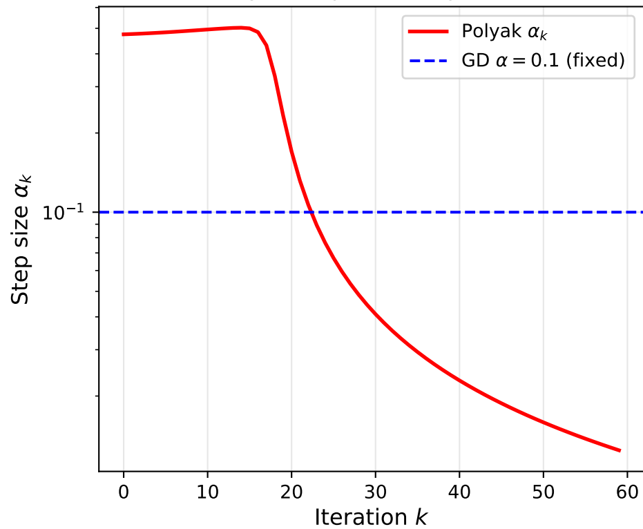
Polyak Step Size Adaptation
