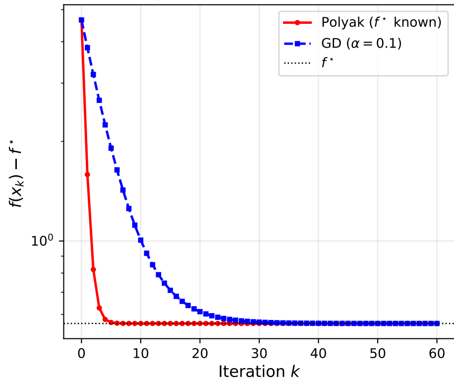
Objective Value (Benchmark A)
