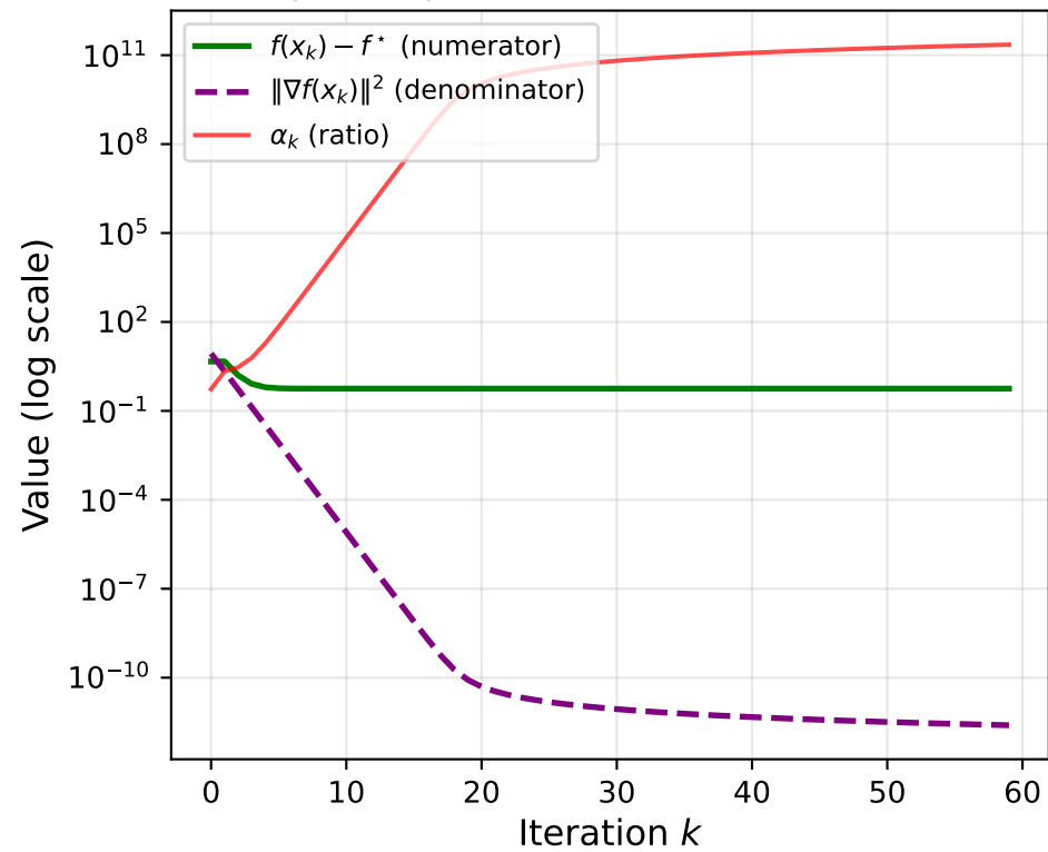
Polyak Step: Numerator vs. Denominator
