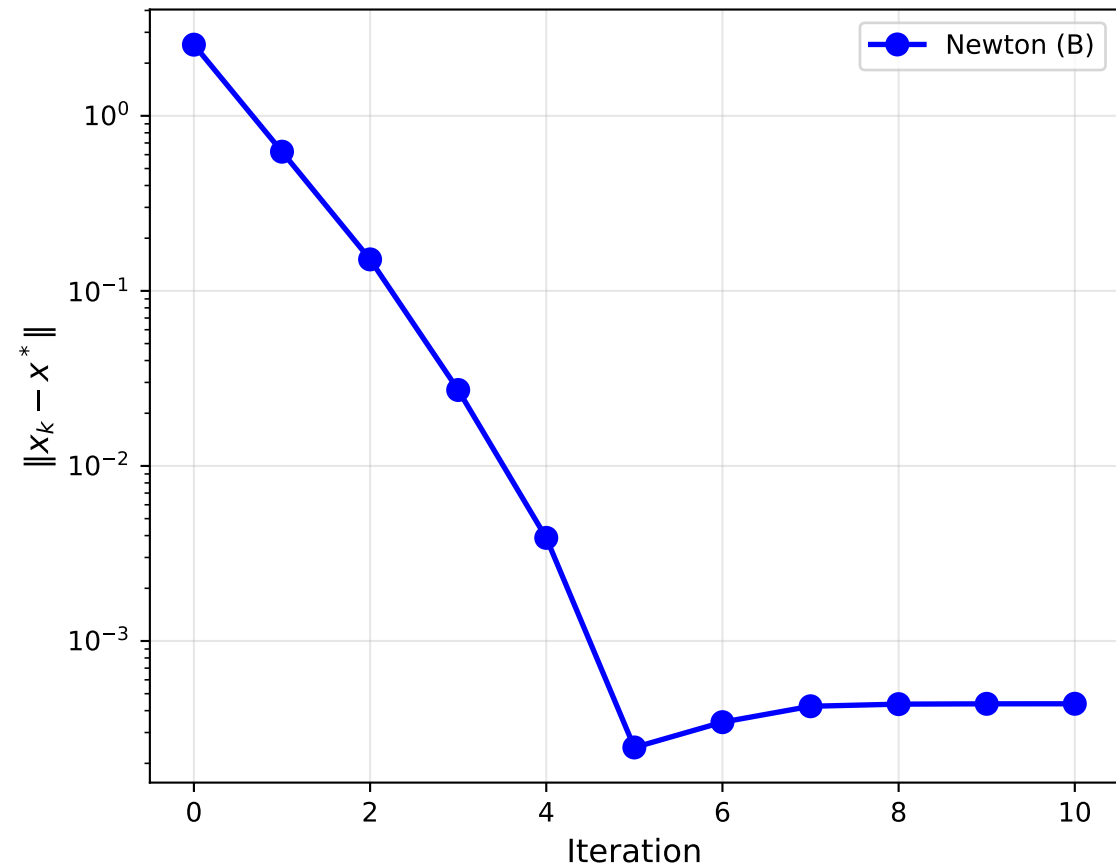
Q3: Newton Convergence on Benchmark B
