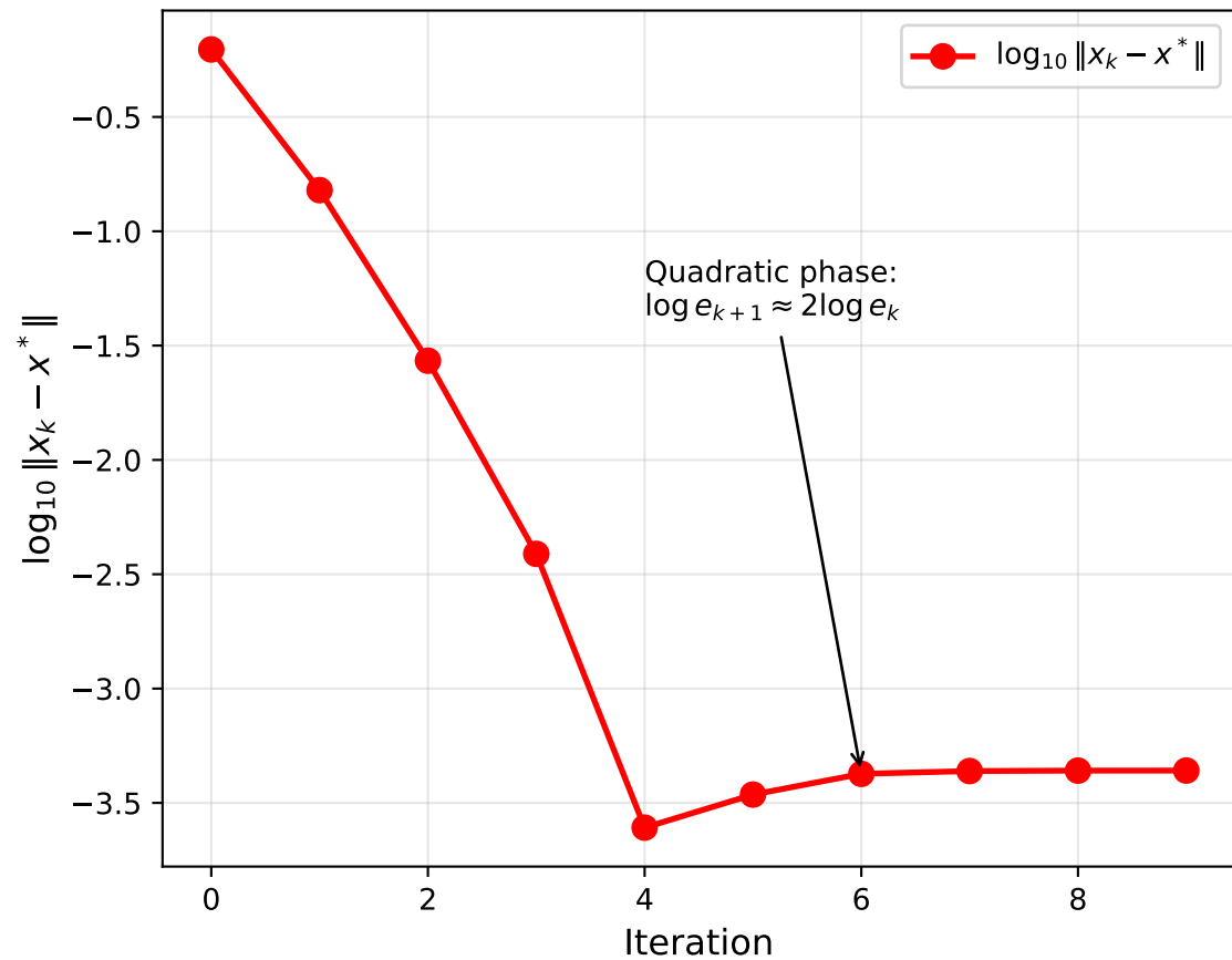
Q3: Log-error -- quadratic convergence phase
