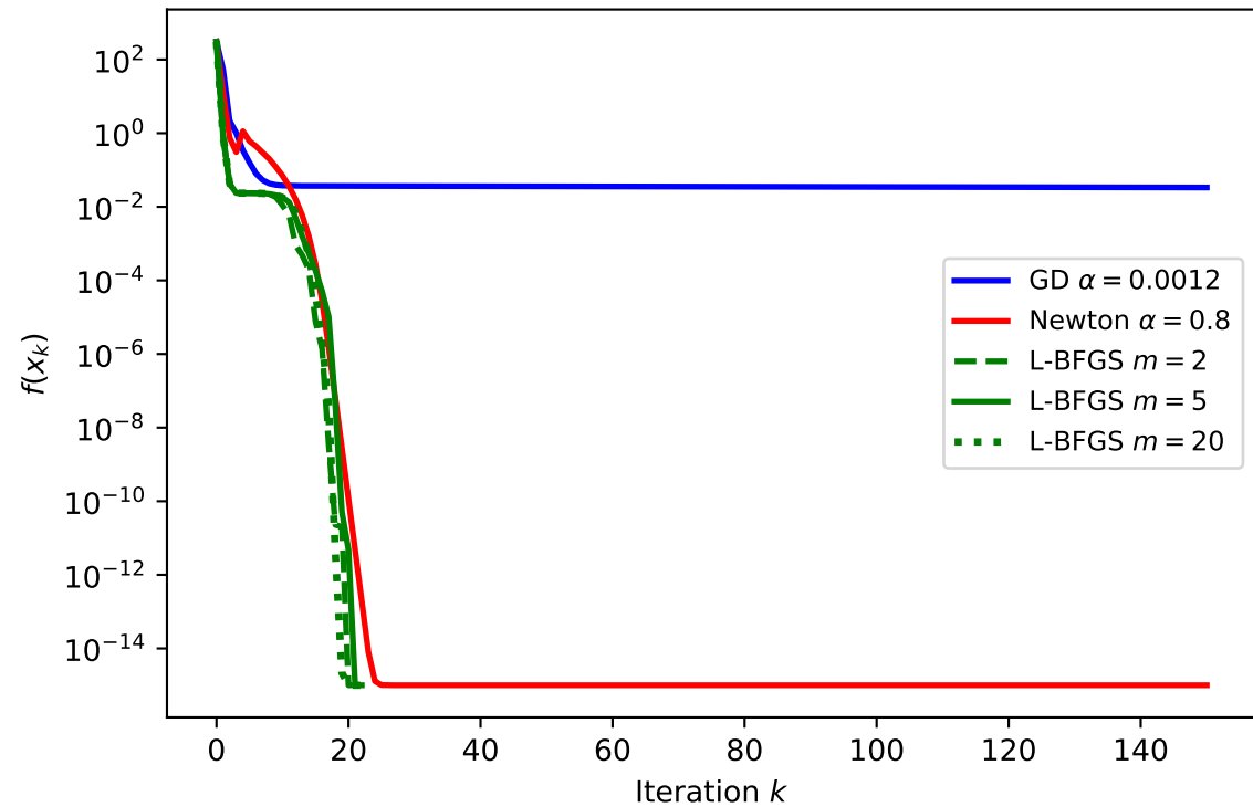
L-BFGS vs Newton vs GD (Rosenbrock, x_0 = (0.5, 2.0) )
