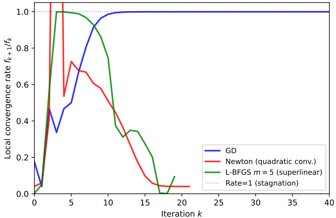
Convergence Rate Analysis (lower = faster convergence)
