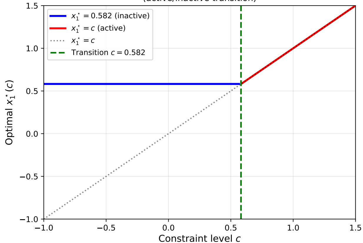
Optimal x_1 vs constraint level (active/inactive transition)
