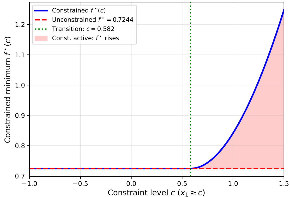
Parametric constraint analysis Optimal value vs c
