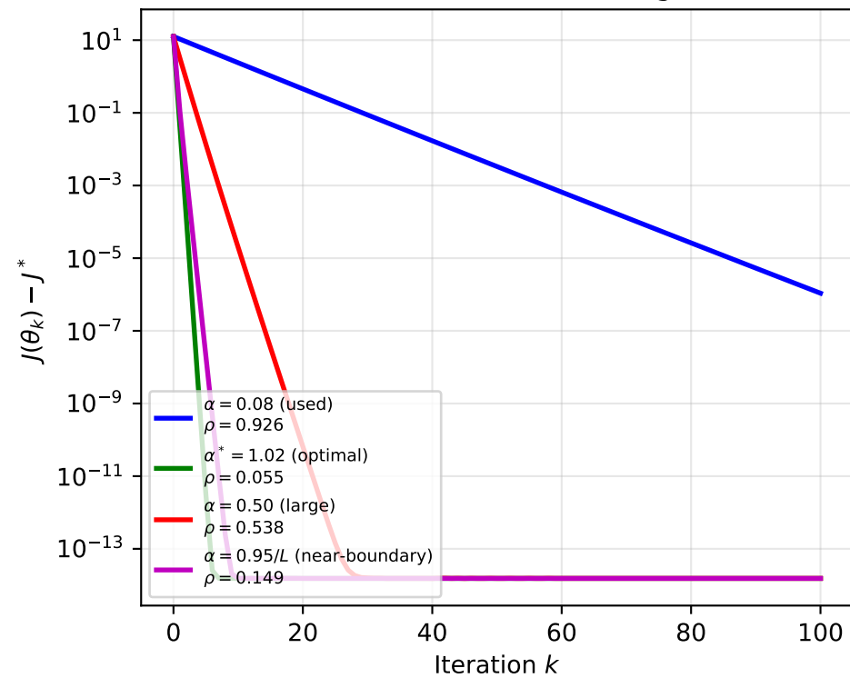
GD Convergence with Different \alpha (Benchmark~A, semi-log)
