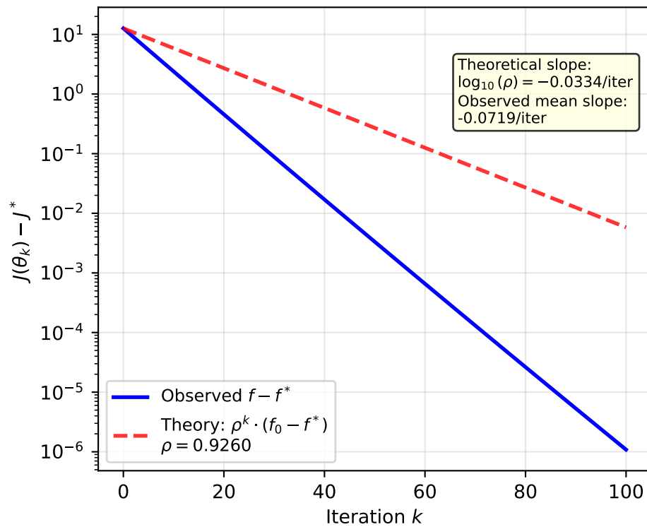
Theory vs Empirical ( \alpha = 0.08 ) Benchmark~A ( \kappa = 1.12 )
