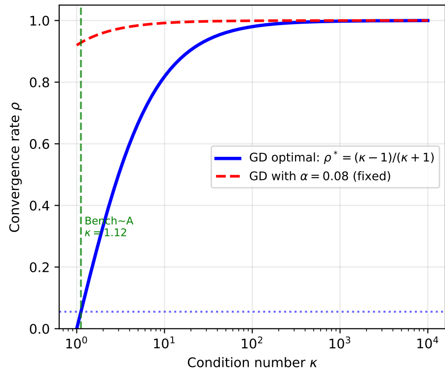
GD Convergence Rate vs \kappa (slower for larger \kappa )
