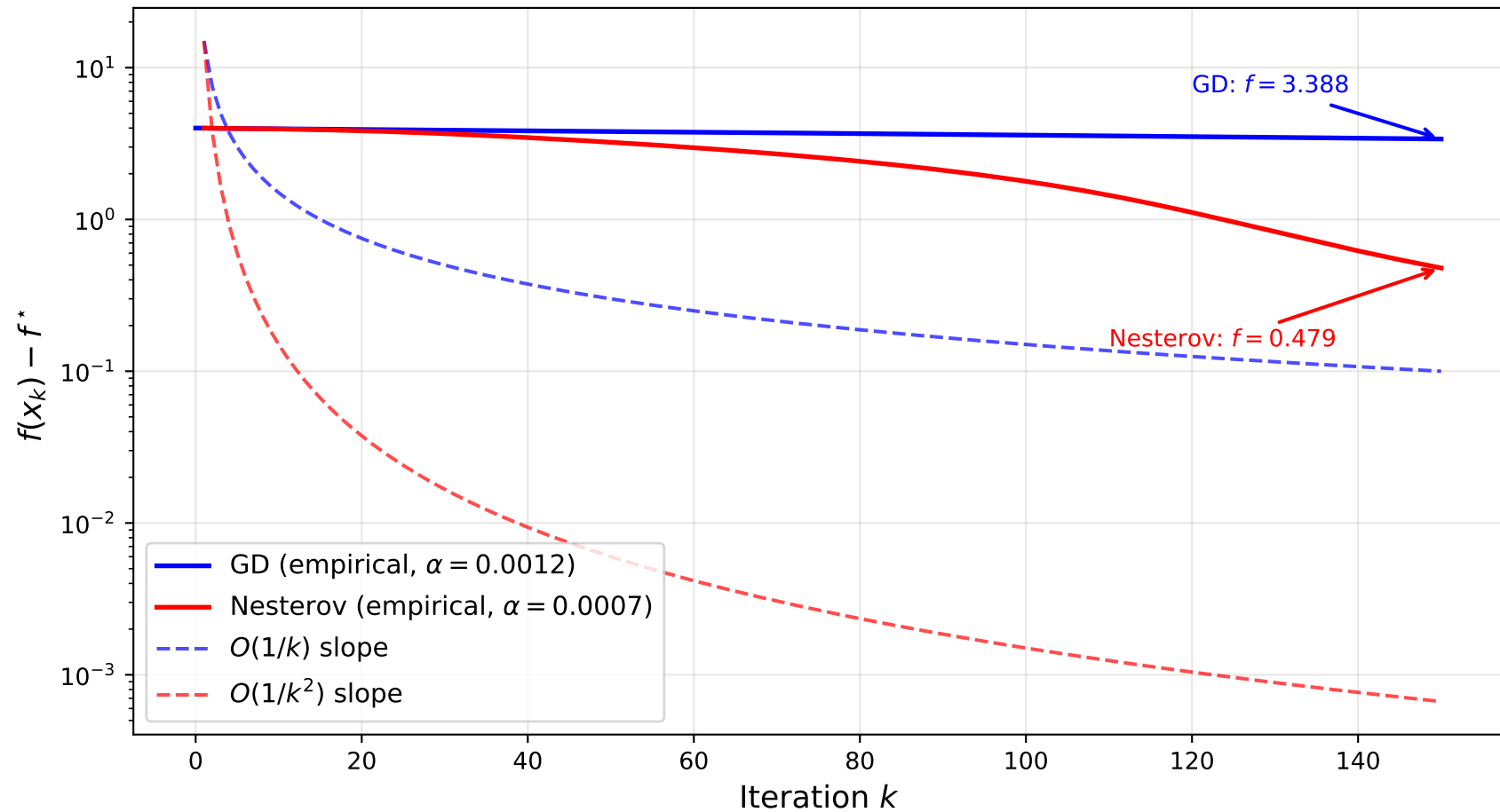
Rosenbrock: Empirical vs Theoretical Convergence Rates (GD O(1/k) vs Nesterov O(1/k^2) )
