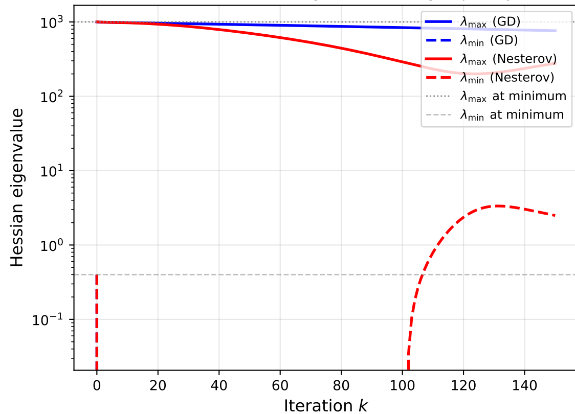
Rosenbrock: Hessian Eigenvalues Along Trajectory
