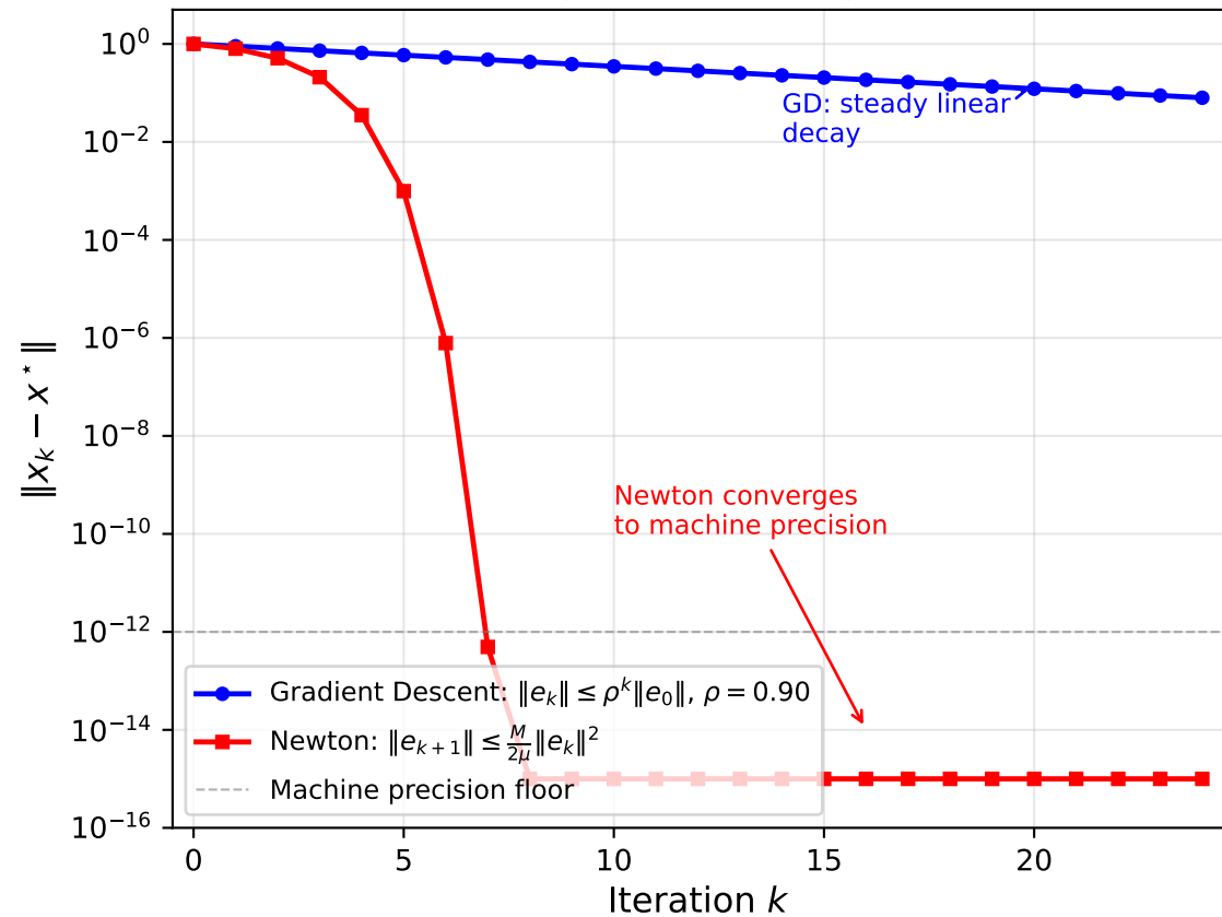
Convergence: Semi-log Scale
