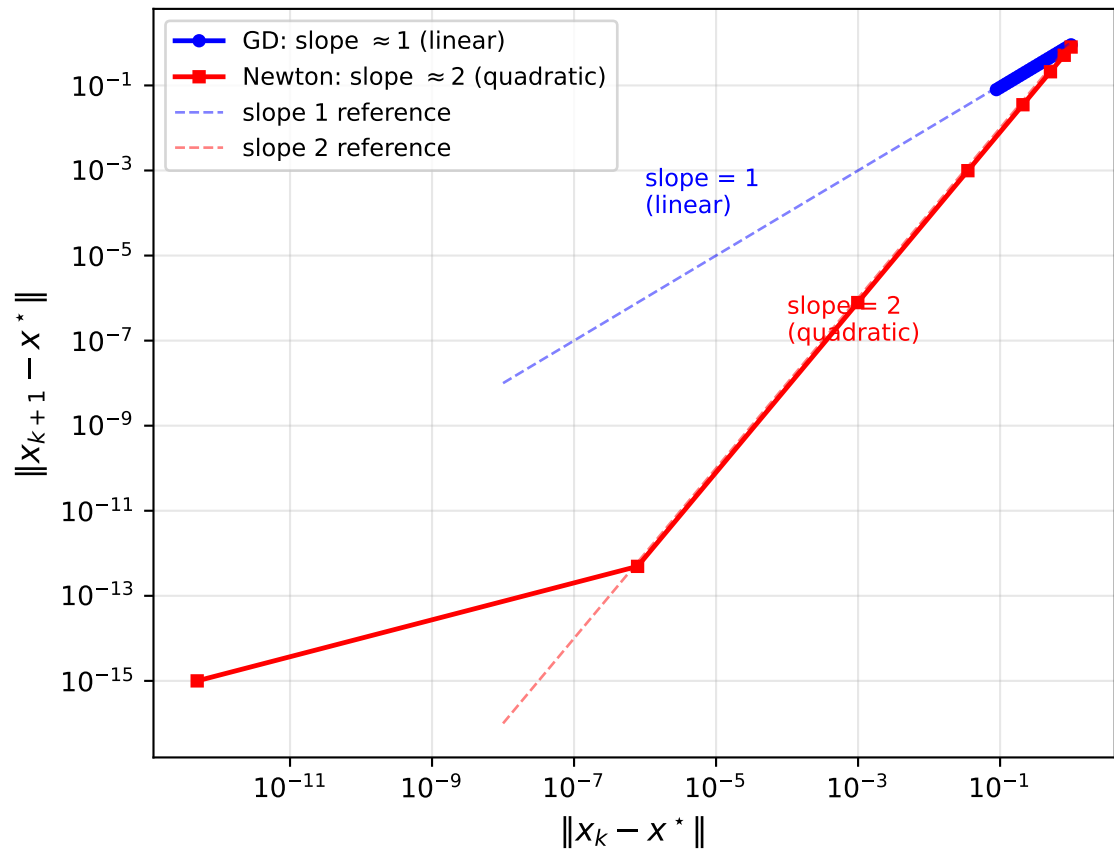
Order-of-Convergence Diagram ( \|e_{k+1}\| vs \|e_k\| )
