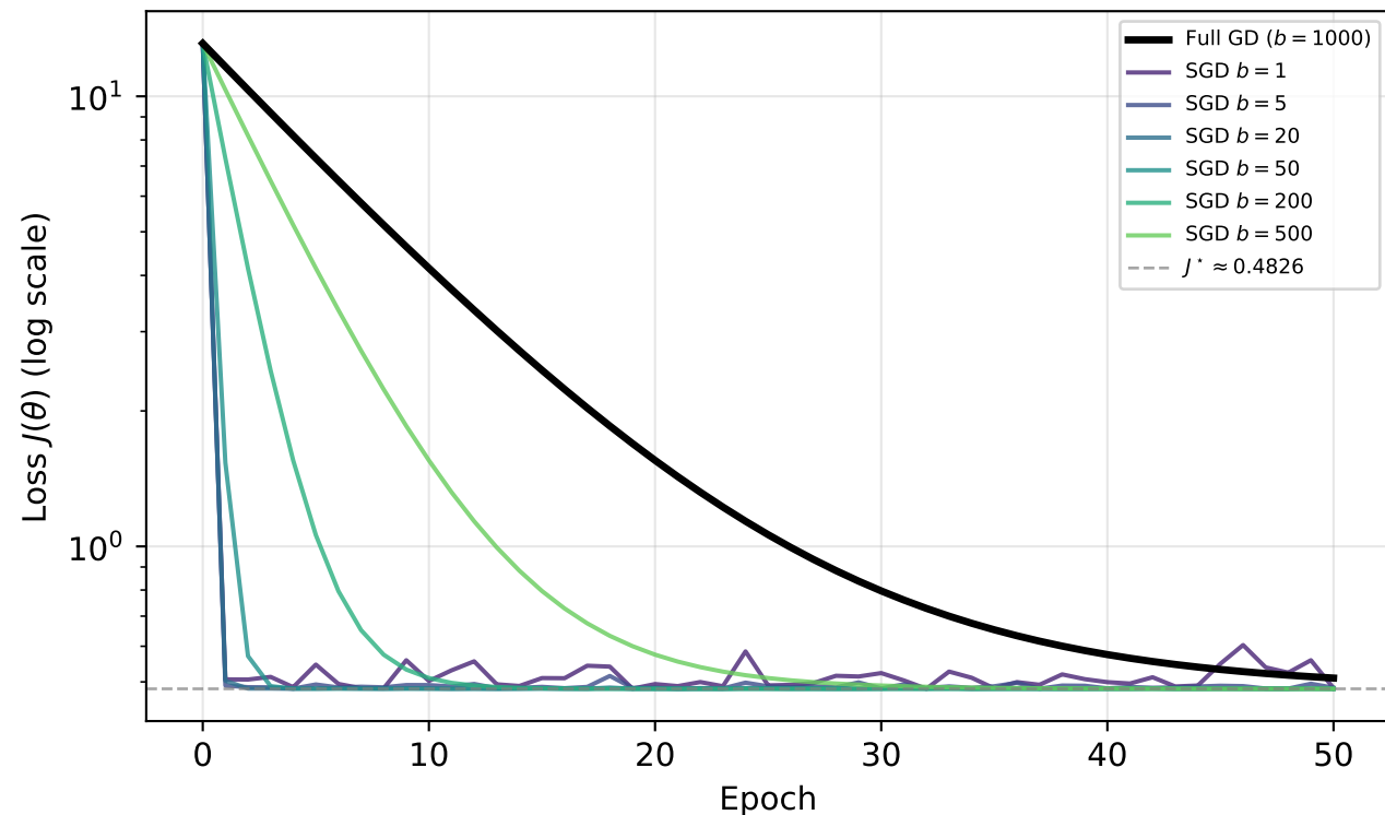
SGD: Per-Epoch Convergence vs Batch Size ( \alpha = 0.06 , Benchmark A)
