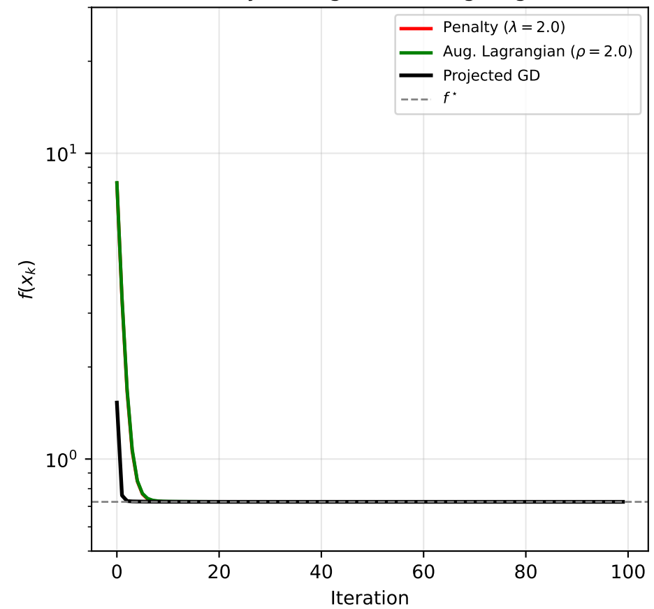
Penalty vs Augmented Lagrangian
