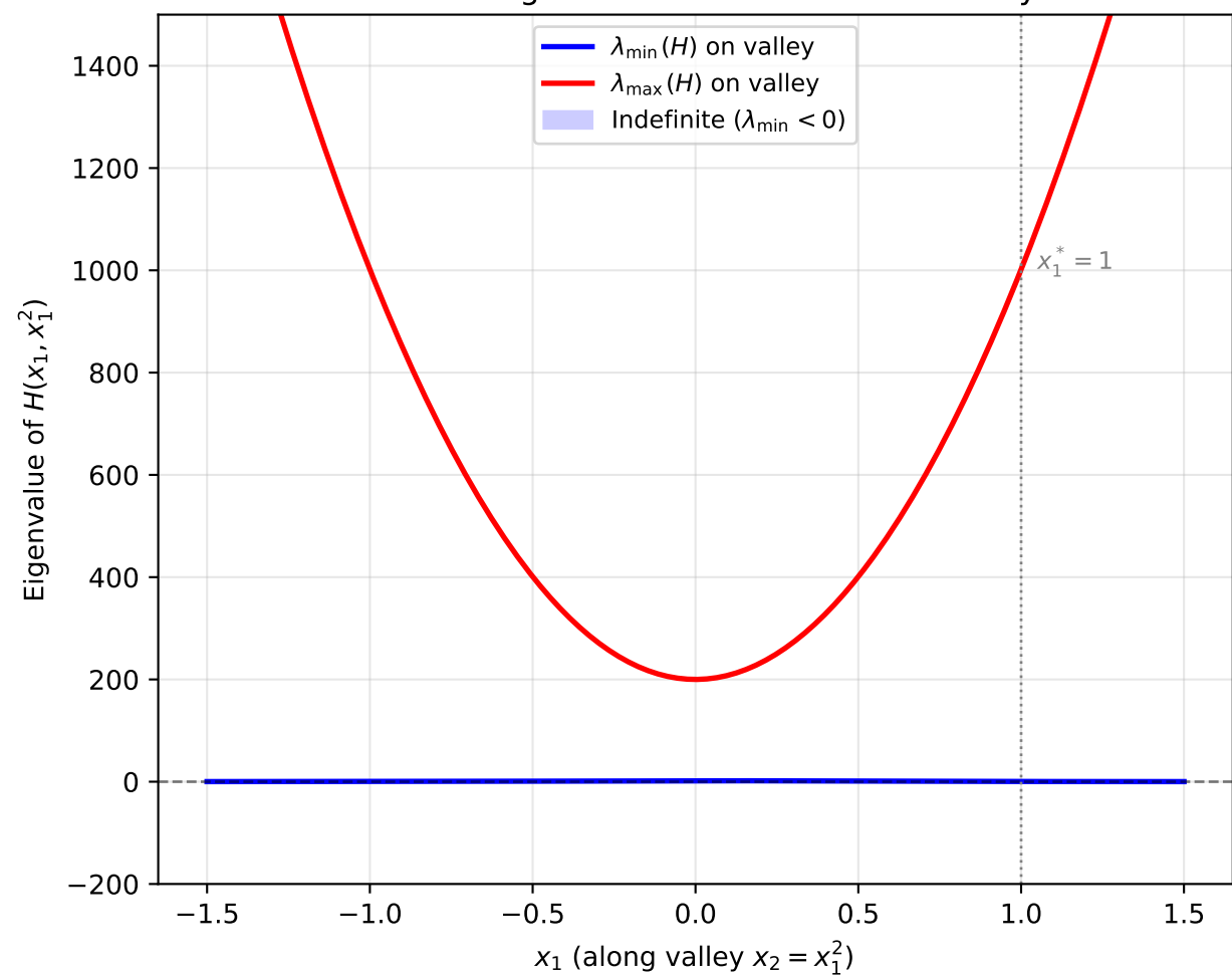
Hessian Eigenvalues on Rosenbrock Valley
