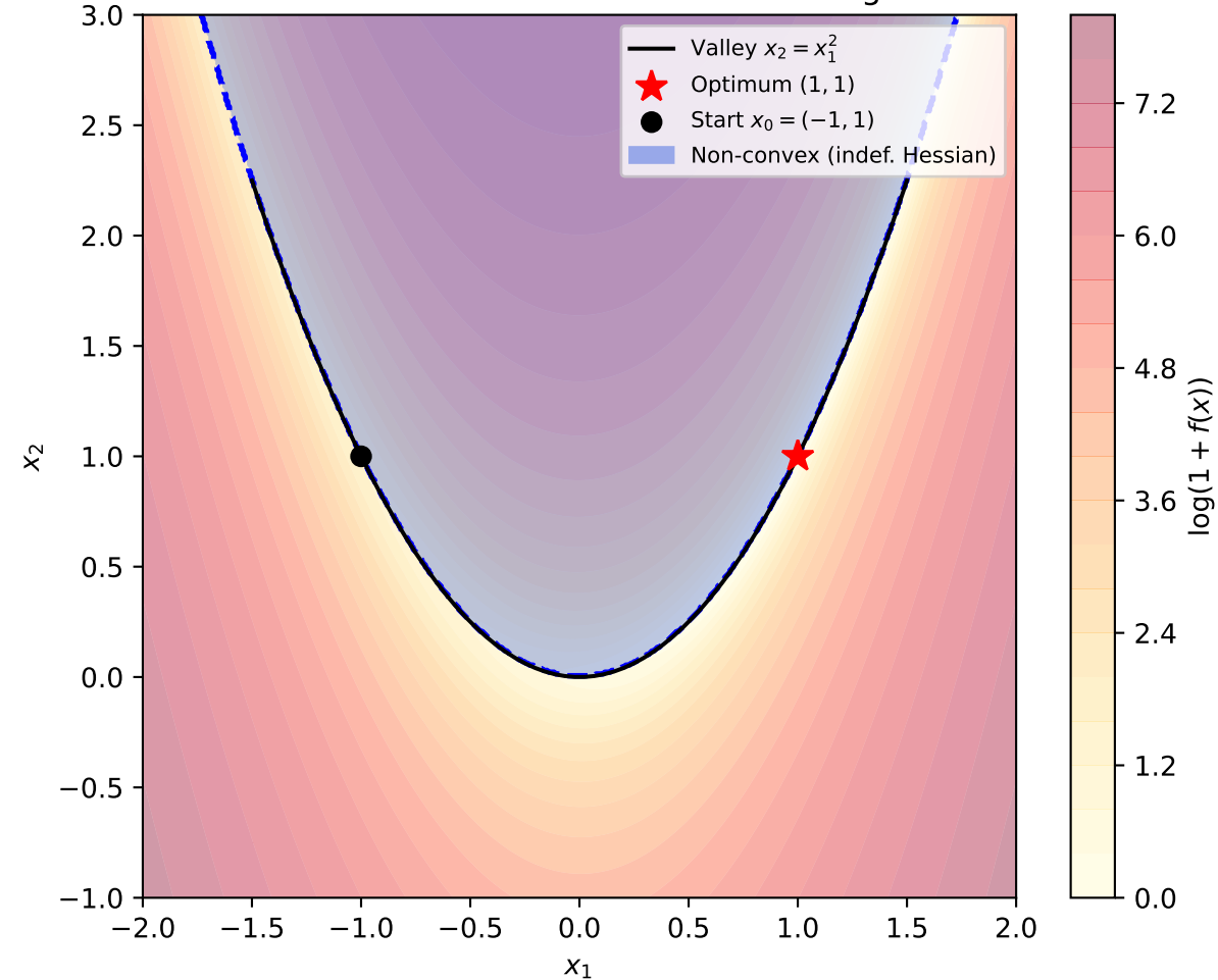
Rosenbrock: Convex vs. Non-Convex Regions
