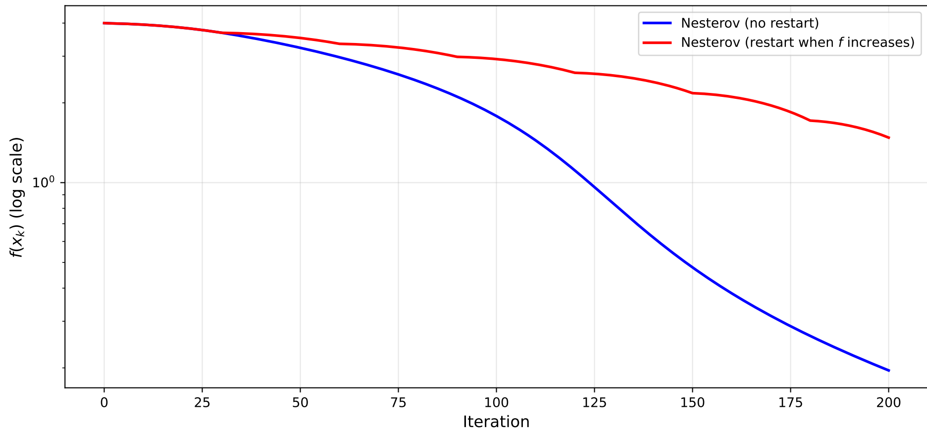
Q2: Nesterov with vs. without Momentum Restart on Rosenbrock
