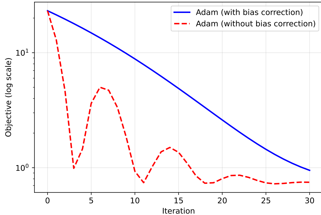
Q2: Effect of Adam Bias Correction (Early iterations, Benchmark B)
