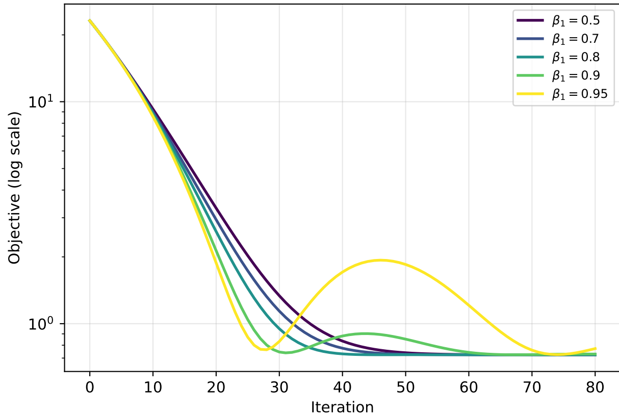
Q2: Effect of \beta_1 on Adam Convergence (Benchmark B, \beta_2 = 0.999 )
