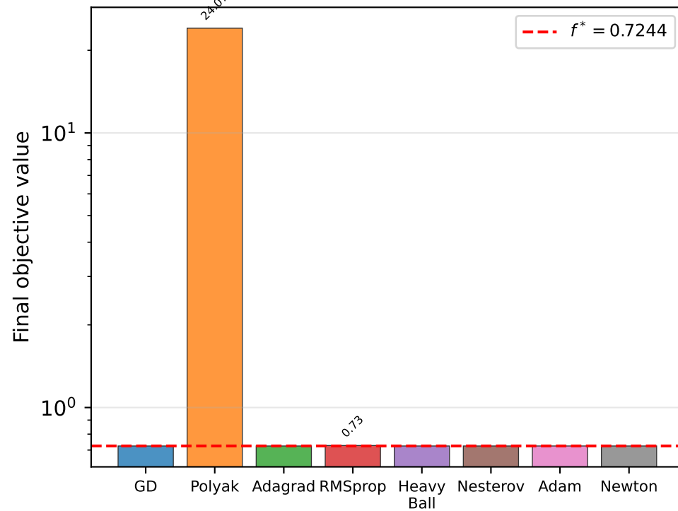
Benchmark B: Toy Neural Network ( \kappa = 6.9 )
