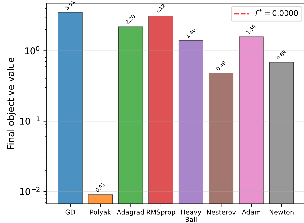
Benchmark C: Rosenbrock ( \kappa = 2508 )
