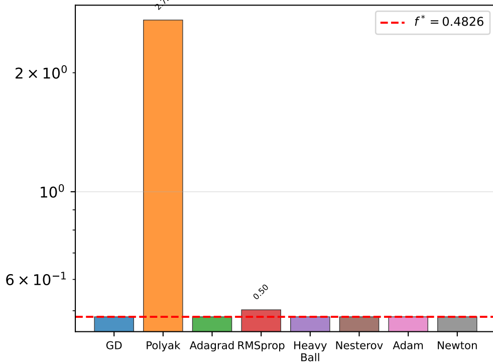
Benchmark A: Linear Regression ( \kappa = 1.12 )
