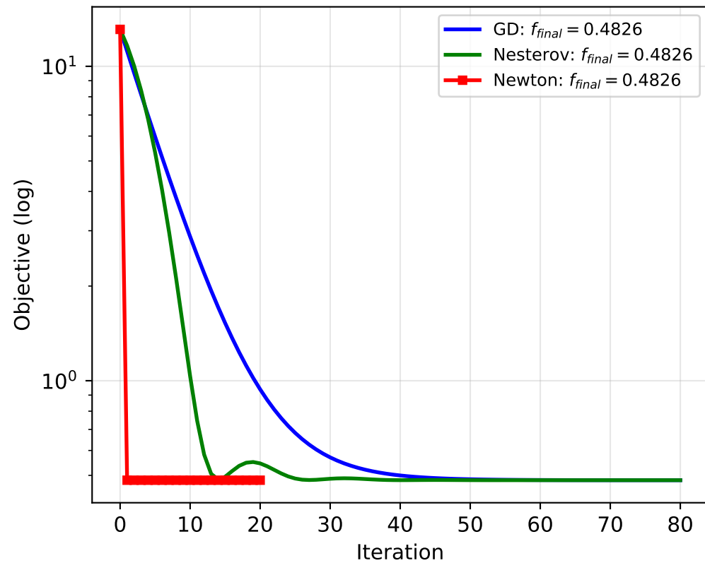
Benchmark A ( \kappa = 1.12 )
