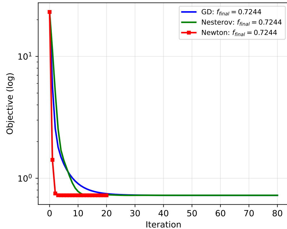
Benchmark B ( \kappa = 6.9 )
