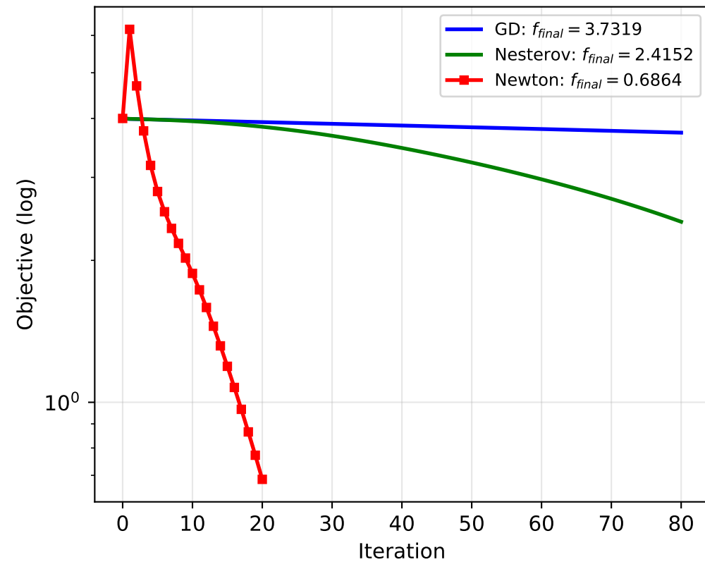
Benchmark C ( \kappa = 2508 )
