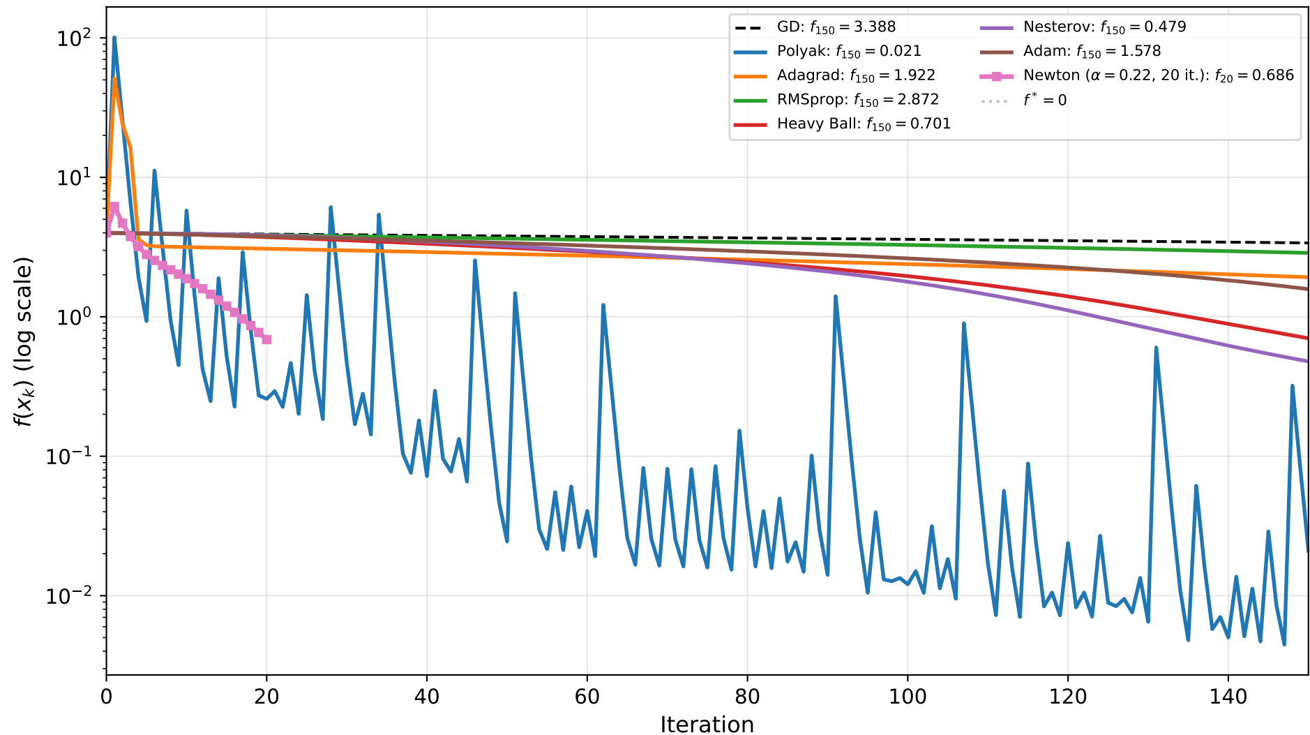
Comprehensive Comparison: All Methods on Rosenbrock ( \kappa \approx 2508 )
